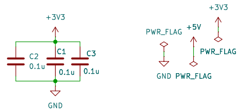
Decoupling Caps (one per IC) and power flags
