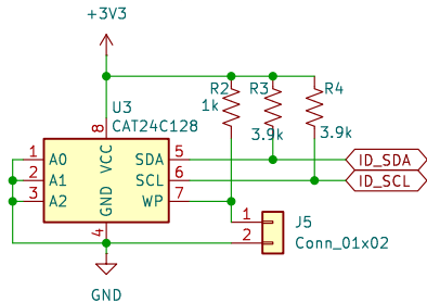
I2C EEPROM (uHat requirement)
