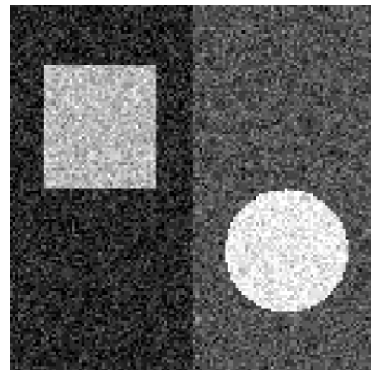
exponential, K=0.2
