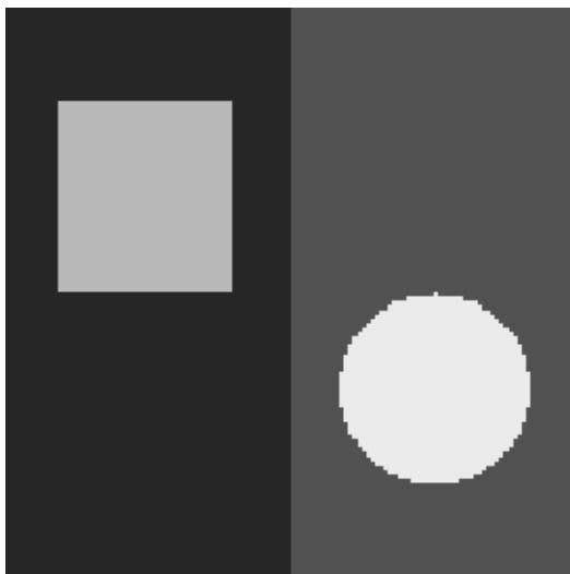
exponential, K=0.05
