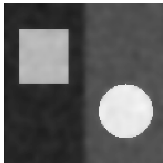
rational, K=0.1
