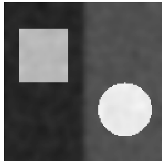
rational, K=0.1
