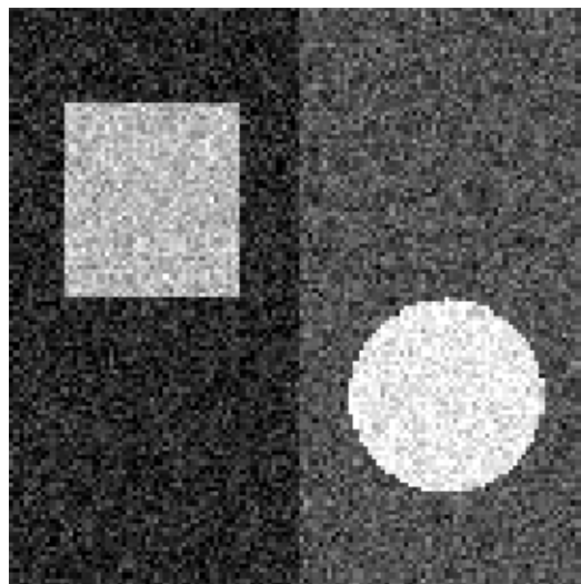
exponential, K=0.1
