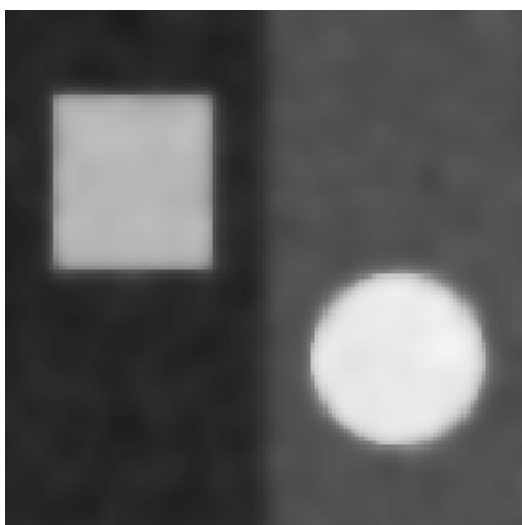
rational, K=0.2
