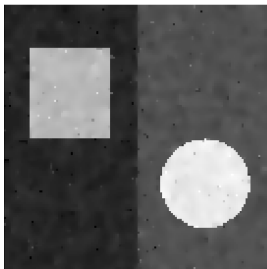
rational, K=0.05
