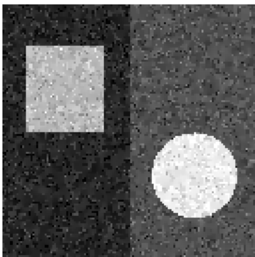
rational, K=0.2
