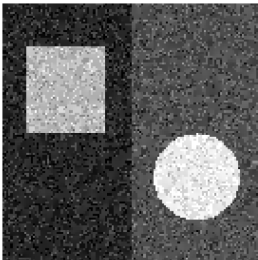
rational, K=0.025
