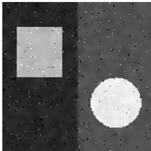
rational, K=0.05
