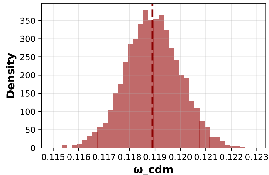
D. CDM Density (Consistent with Planck)
