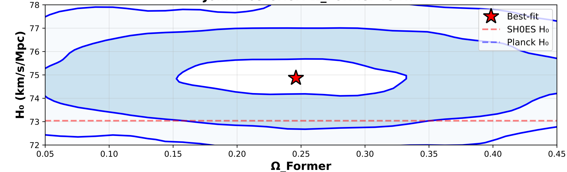
F. Joint Posterior: \Omega_{\text{Former}} vs H_0
