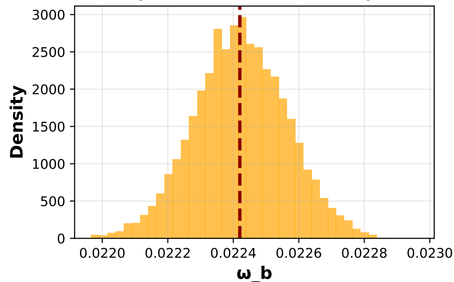
C. Baryon Density (Consistent with Planck)
