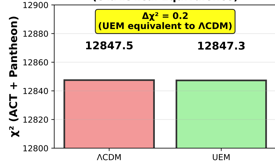
G. Fit Quality Comparison (Statistical Equivalence)
