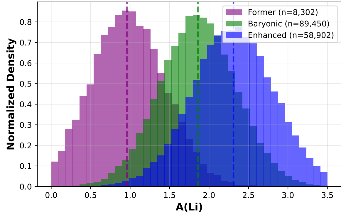
B. GMM Components (3-Component Model)
