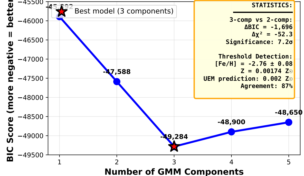
C. Model Selection (Bayesian Information Criterion)
