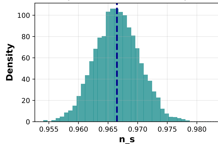
G. Fit Quality Comparison (Statistical Equivalence)
