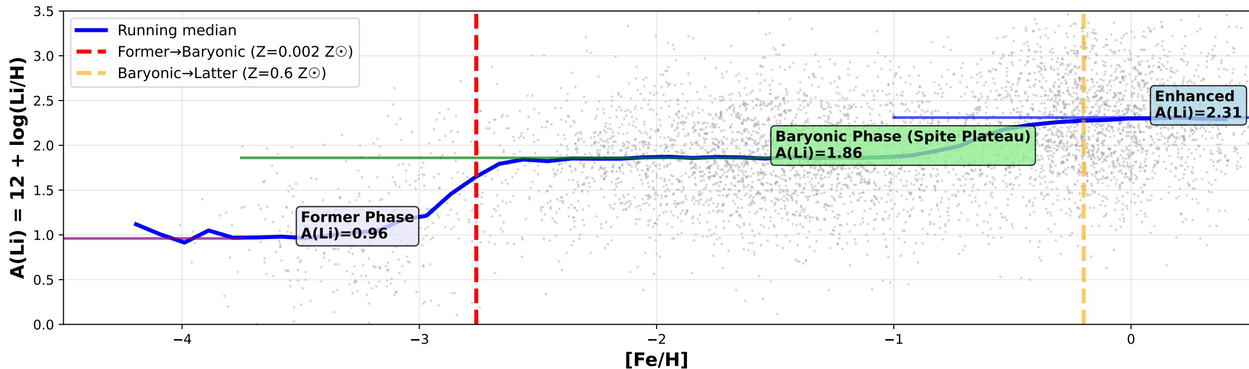
A. Lithium Abundance vs Metallicity (GALAH DR3, n=156,656 stars)
