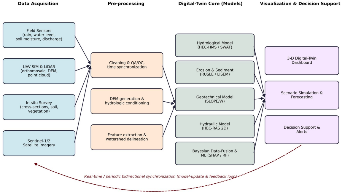
Fig. 5. Digital-twin architecture and data pipeline: data acquisition, pre-processing, digital-twin core models, and visualisation and decision support, linked by a real-time/periodic bidirectional model-update and feedback loop.
