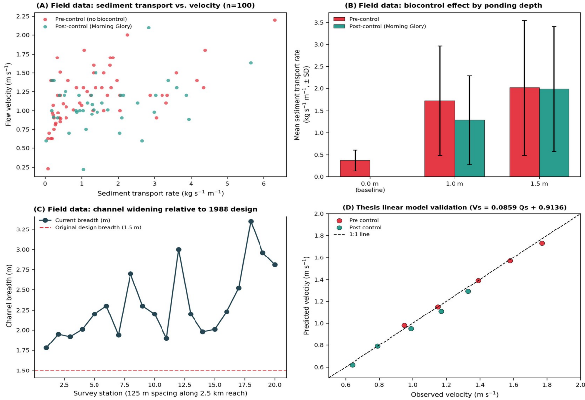
Fig. 4. Field-measured validation dataset from the author's 2024 undergraduate field trial at the ABU Dam watercourse (n=100 records): (A) sediment transport rate vs. flow velocity, pre- vs. post-control; (B) mean sediment transport rate ( \pm SD) by ponding depth and control status; (C) surveyed channel breadth at 20 stations vs. the 1988 original design breadth; (D) validation of the thesis's own linear regression model (Eq. (1)) against observed velocities, pre- and post-control.
