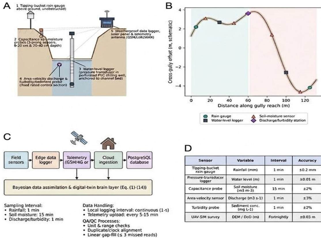
Fig. 3. Sensor installation and data-recording architecture: (A) physical structure of a gully monitoring station showing the installed instruments – tipping-bucket rain gauge, three-prong capacitance soil-moisture probes, perforated-PVC stilling well with pressure-transducer water-level logger, area-velocity/turbidity probe, and the weatherproof data-logger enclosure with solar panel and telemetry antenna; (B) monitoring network layout along the treated and untreated reaches; (C) five-stage data-recording and telemetry architecture from field sensor to Bayesian digital-twin assimilation; (D) sensor sampling configuration, intervals and manufacturer-stated accuracy.
