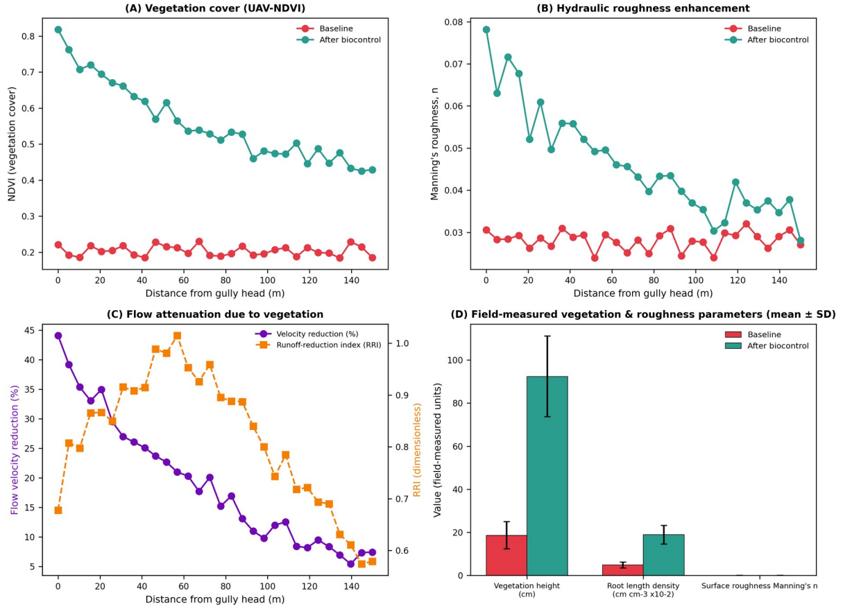
Fig. 10. Biocontrol effectiveness of Morning Glory ( Ipomoea spp.): (A) NDVI vegetation cover, (B) Manning's roughness coefficient, (C) flow-velocity reduction and Runoff-Reduction Index, and (D) paired field measurements of vegetation height, root density and roughness (mean \pm SD).
