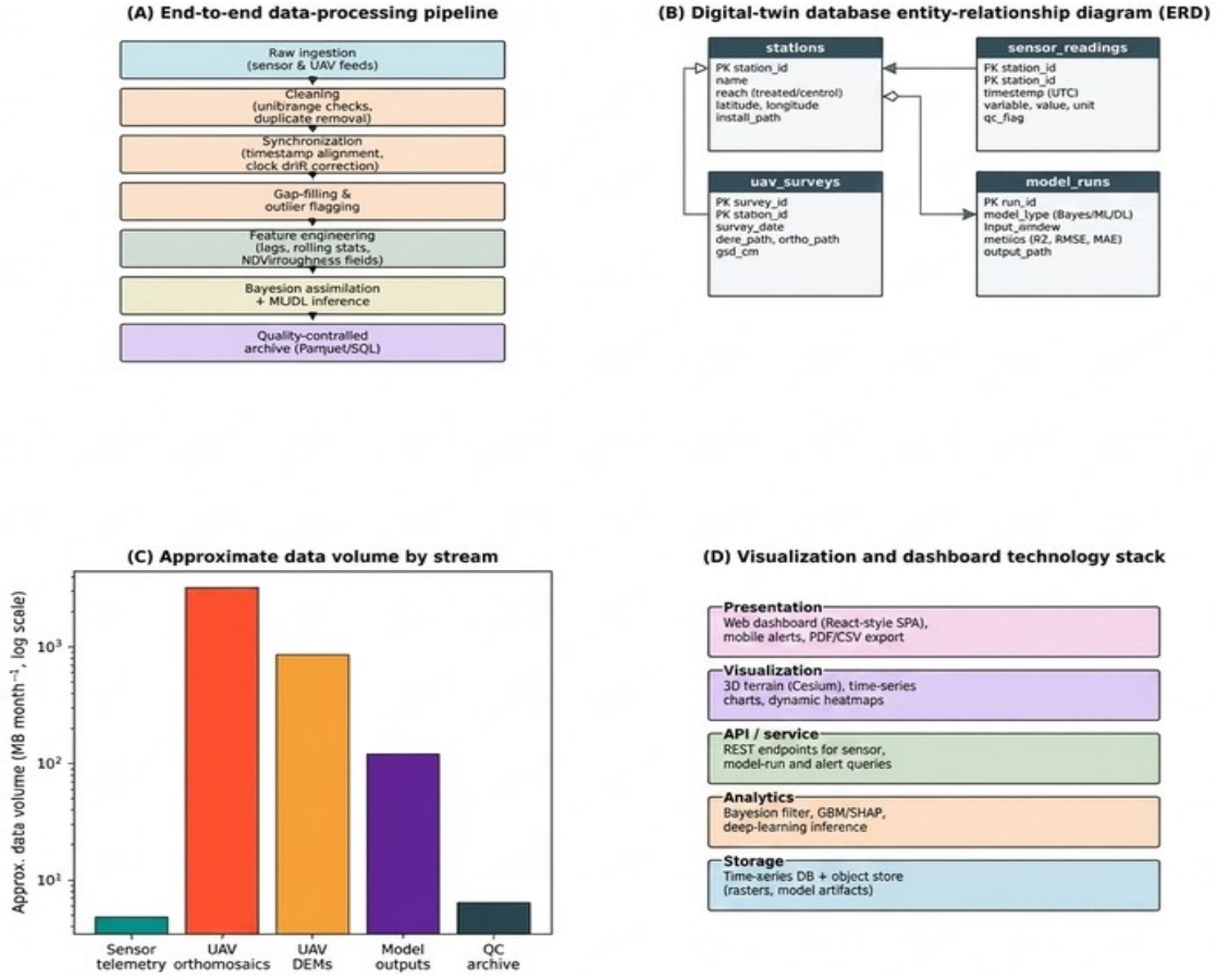
Fig. 6. Data processing, storage and visualization architecture: (A) end-to-end data-processing pipeline; (B) digital-twin database entity-relationship diagram; (C) approximate monthly data volume by stream; (D) visualization and dashboard technology stack.
