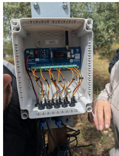
Inspecting a LoRa IoT irrigation sensor box in the field, 2025
