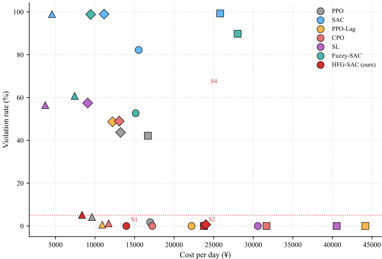
Cost-safety Pareto frontier (mean of 3 seeds)
