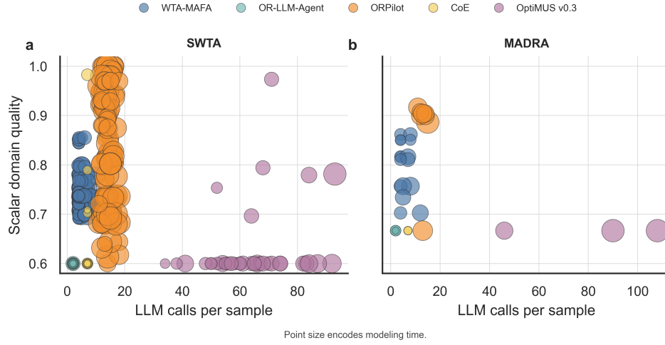
Figure E1 Per-sample LLM calls versus scalar domain quality on SWTA (a) and MADRA (b); point size encodes modeling time. Each point is one scored output, including outputs that fail public feasibility. Every publicly feasible SWTA output of CoE and OptiMUS v0.3 is an empty plan scoring 0.600 (Table E3), so their SWTA points above 0.600 are outputs that fail public feasibility; ORPilot’s SWTA points include the 85 outputs whose untimed plans fail the time-indexed checks. The MADRA points of OR-LLM-Agent, CoE and OptiMUS v0.3 at 0.667 are empty plans.
