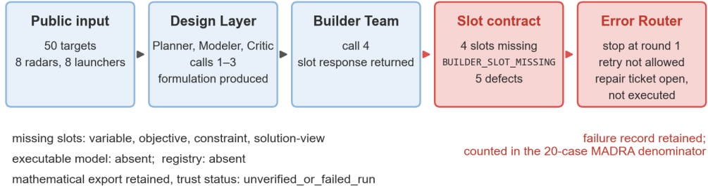
Figure J1 Case II: MADRA trace stopped at the first route decision.
