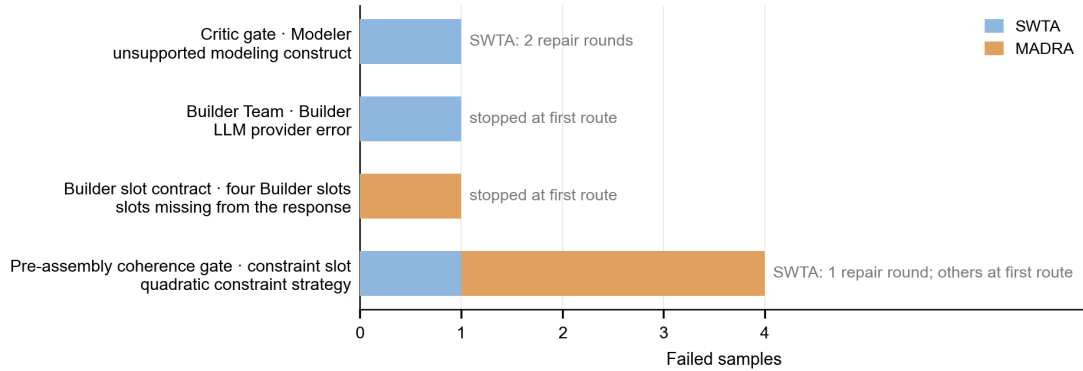
Figure E2 Where the seven WTA-MAFA failures stop, by gate and responsible component; numbers give the repair rounds completed before the stop.
