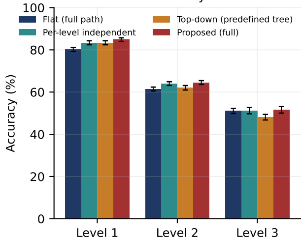
Accuracy
