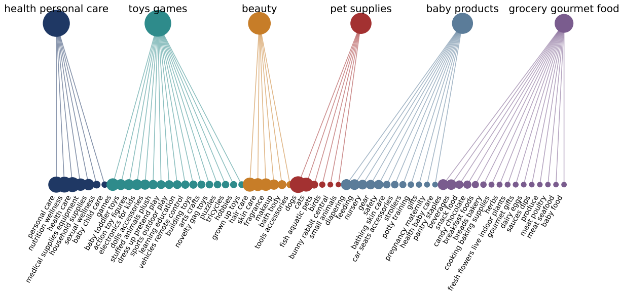
Reference label structure: 6 level-1 categories over 64 level-2 categories (node area proportional to document frequency)
