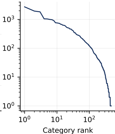
Level 3 (473 classes)
