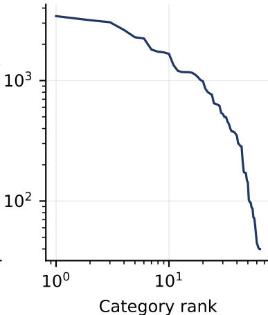
Level 2 (64 classes)
