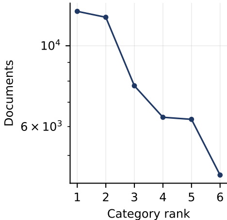
Level 1 (6 classes)
