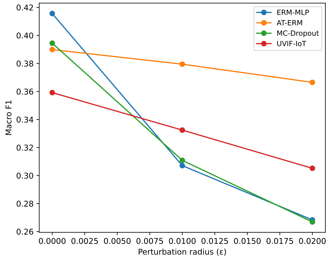
PGD Robustness — UNSW
