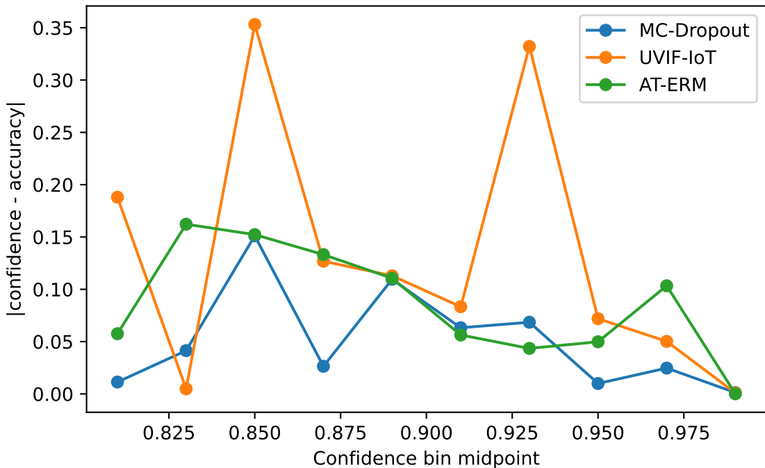
High-Confidence Calibration Gap — NBAIoT
