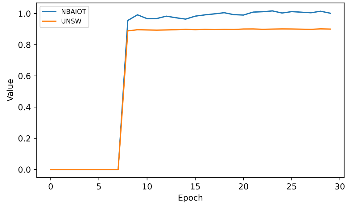
Calibration
