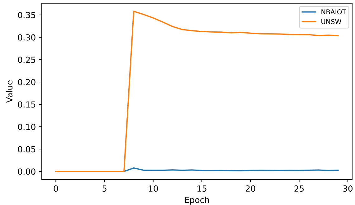
Calibration
