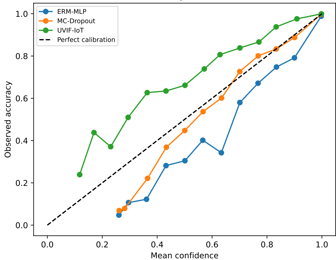
Reliability — UNSW
