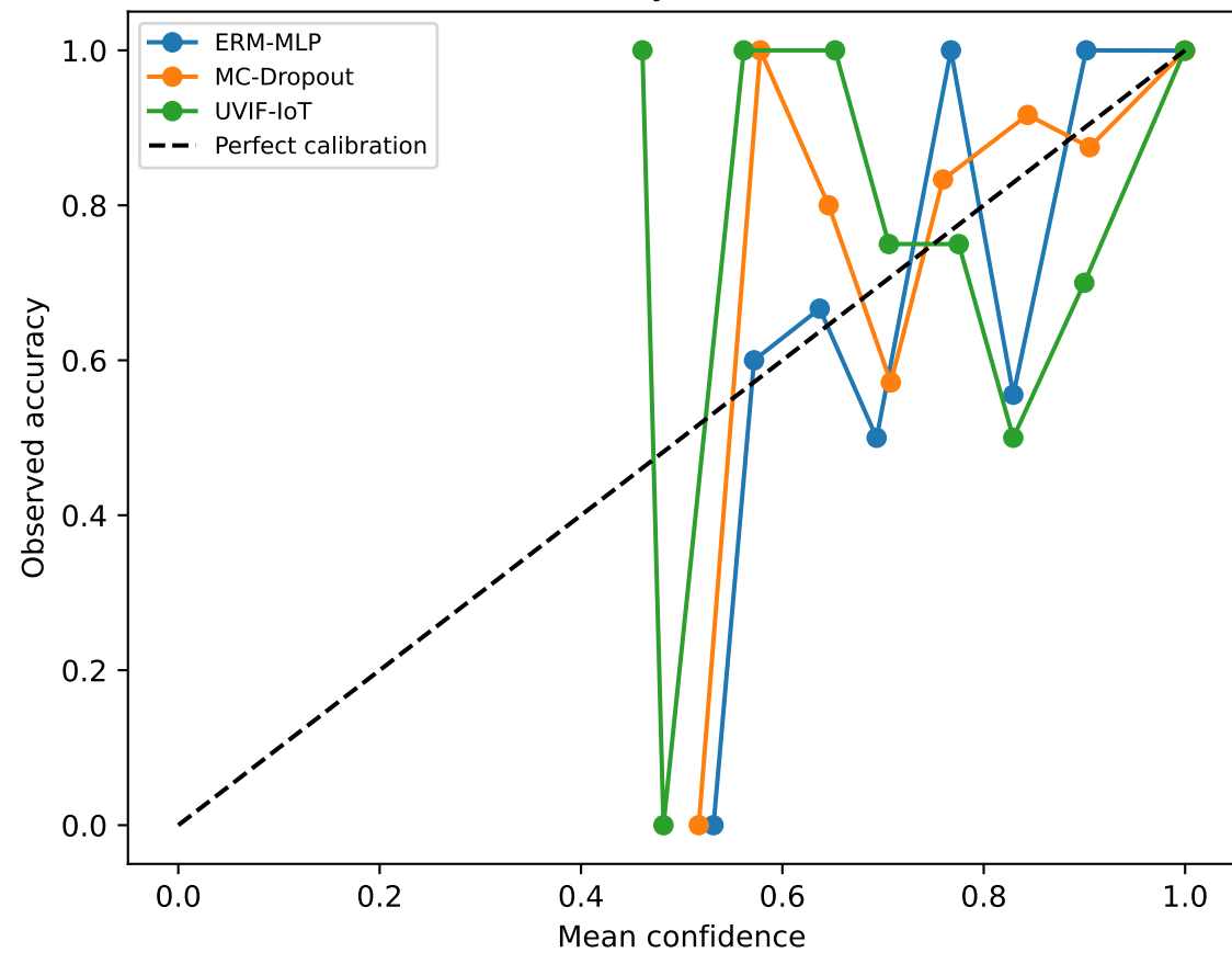
Reliability — NBAIoT
