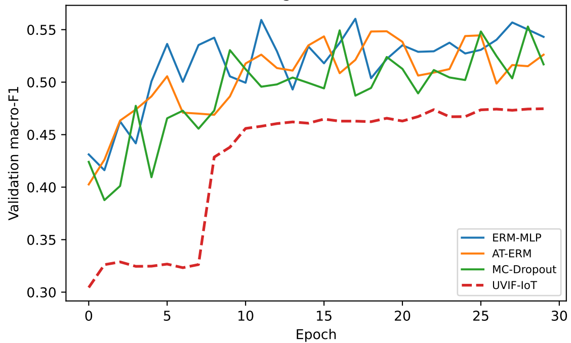
Convergence — UNSW
