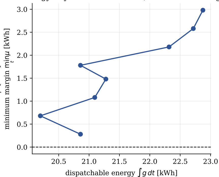
Within the certified subset ( \bar{\mu} \geq 0.2 ): energy buys interior distance, not less shedding
