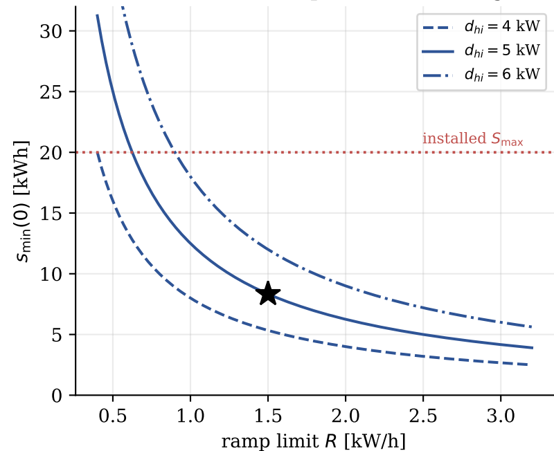
Slow actuation is paid for in storage
