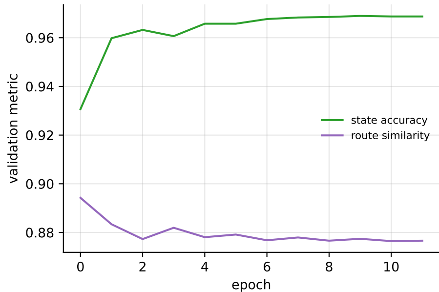
Validation
