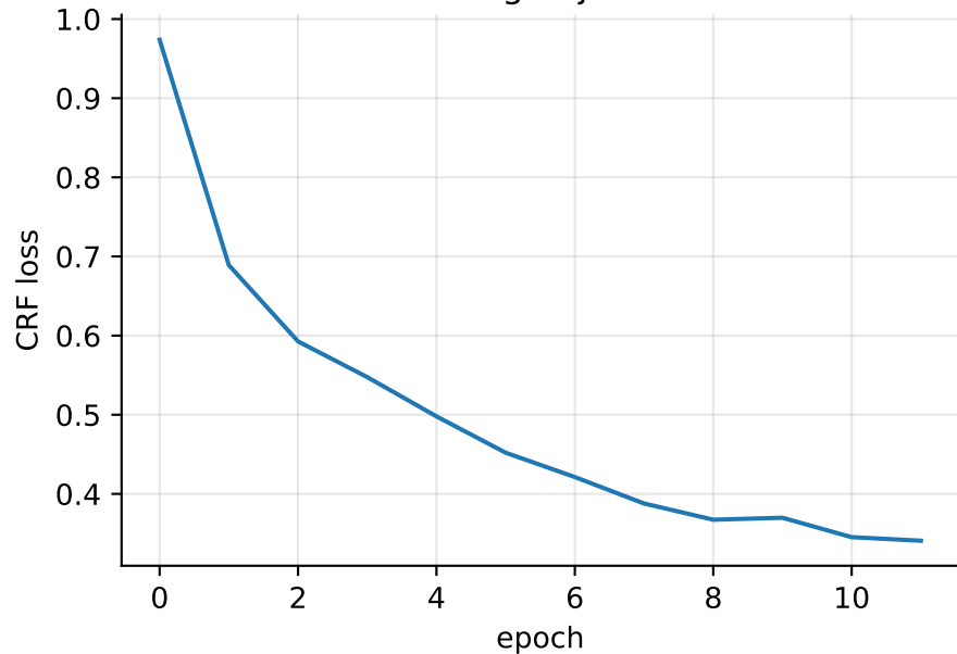
Training objective
