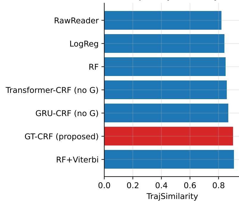
Trajectory similarity
