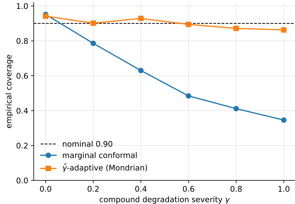
Coverage under distribution shift
