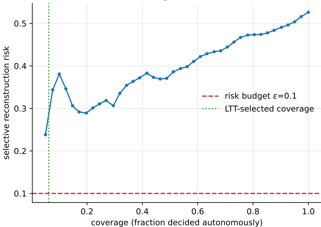
Risk-coverage (AURC=0.399)
