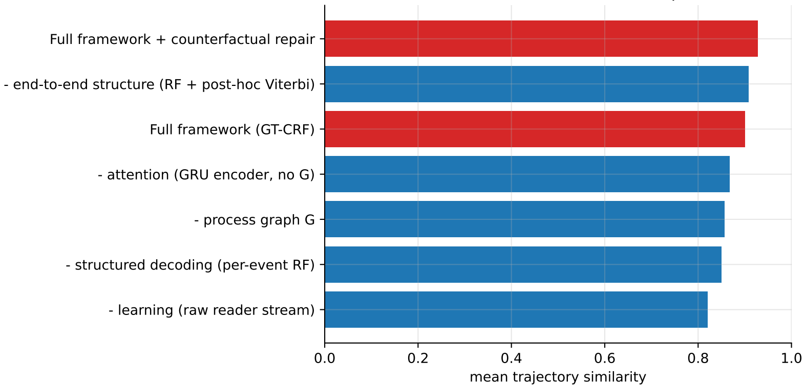
Ablation: contribution of each component
