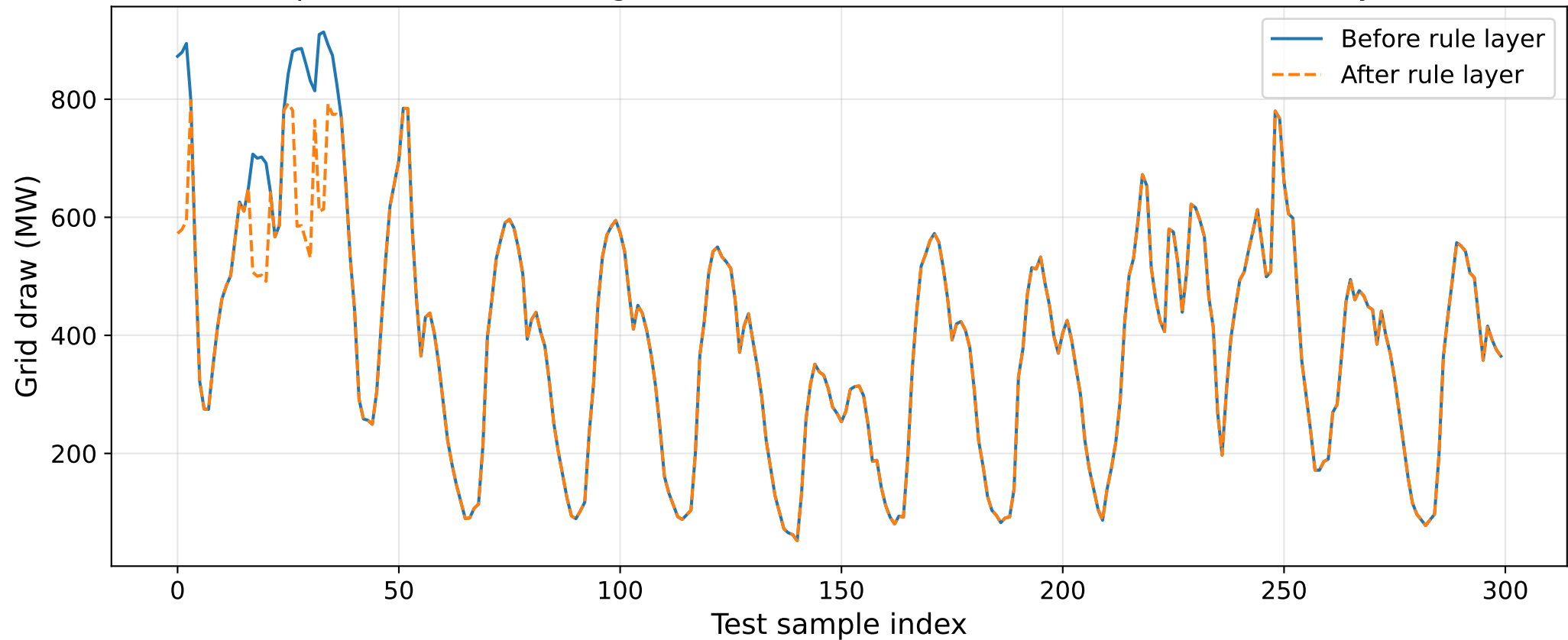
Operational scenario: grid draw before and after rule-based decision layer
