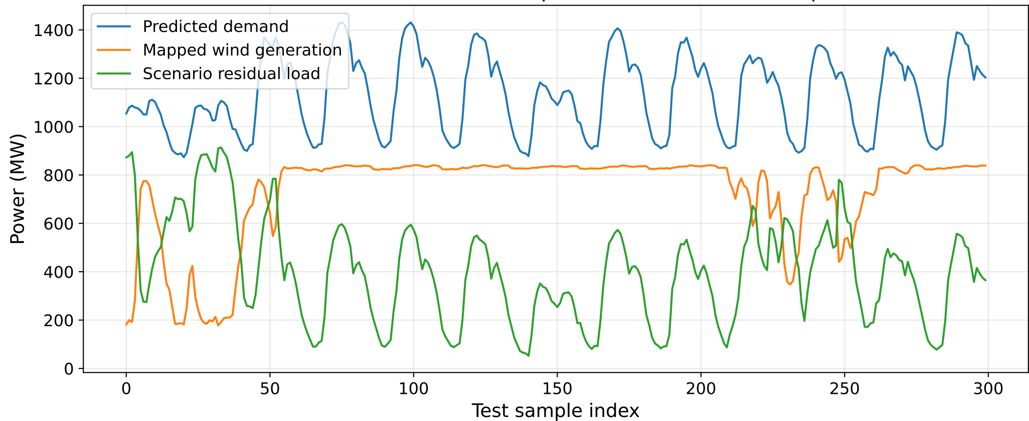
Scenario-based residual-load computation from coordinated predictors
