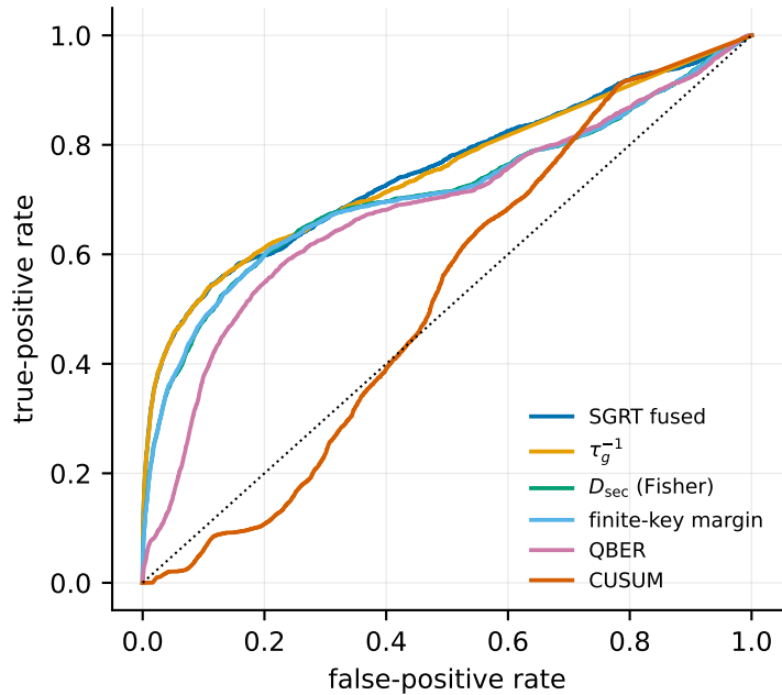
(a) ROC — collapse within H = 30 blocks
