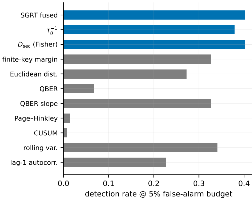
(a) episode detection
