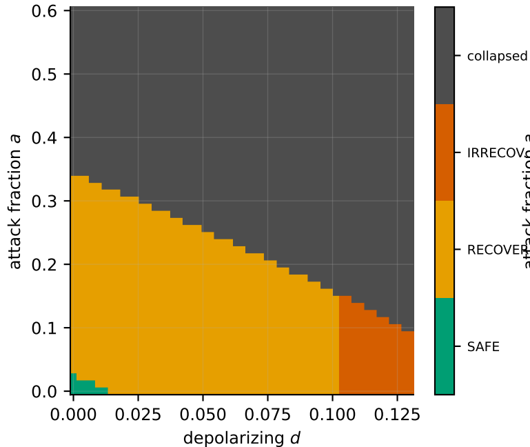
(a) viability classes ( \phi = 0.005 , H_c = 60 )
