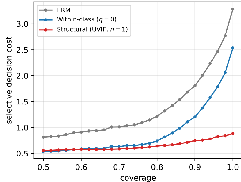
H1: risk-coverage under shift ( \delta = 3 )
