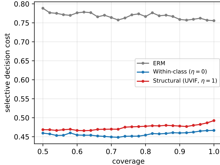
In-distribution ( \delta = 0 ): near-equivalence
