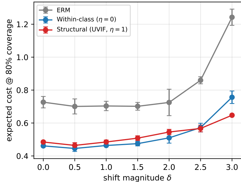
H3: dose-response of the structural advantage
