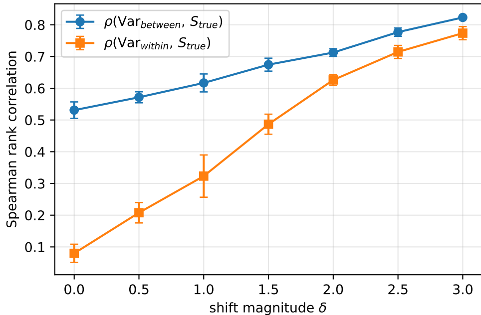
H2: tracking of ground-truth structural error
