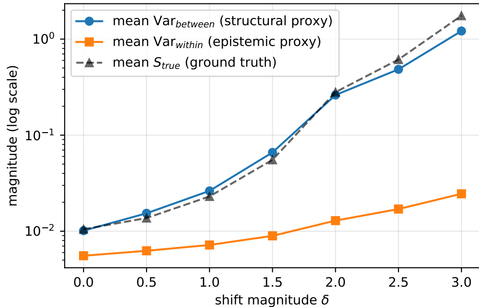
Growth of the components under shift
