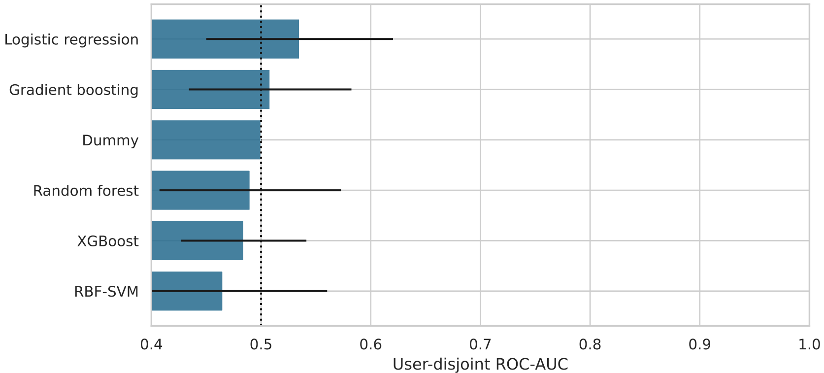
Figure 4. Leakage-controlled classifier comparison
