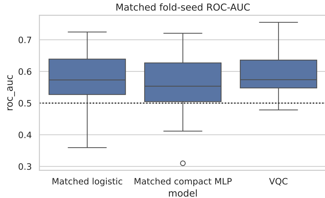
Figure 8. Matched quantum-classical classification
