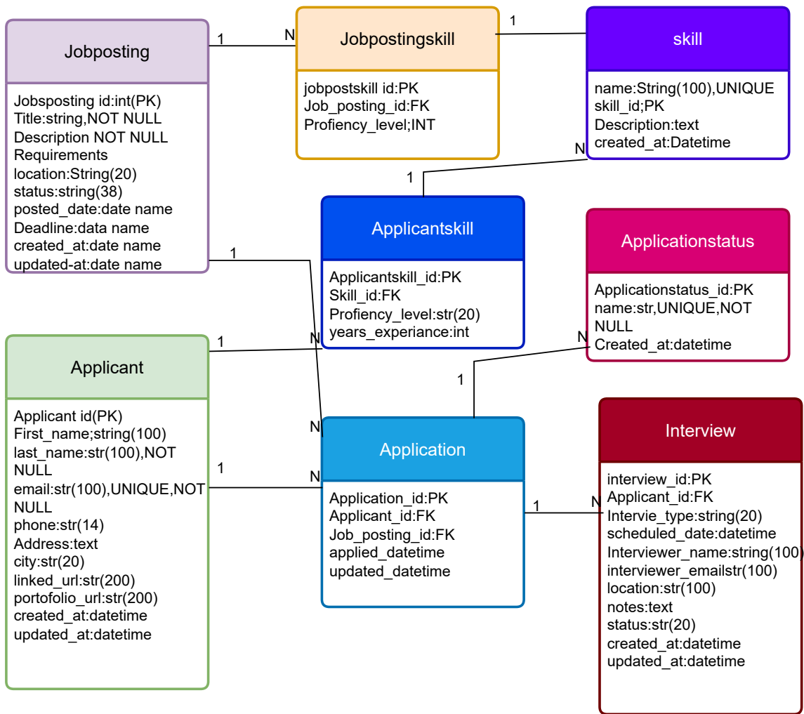
Job ApplicationTracking System-Entity Relationship Diagram
