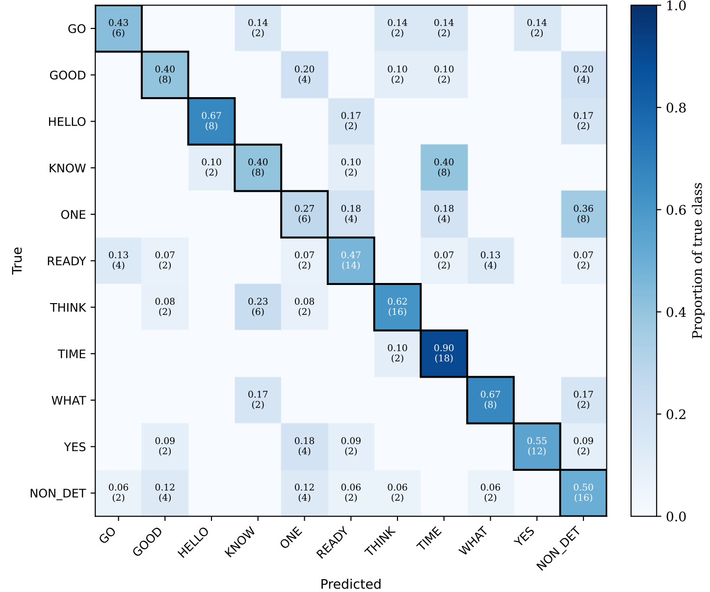
NON_DETECTION v3 (235 test clips, 11 classes)
