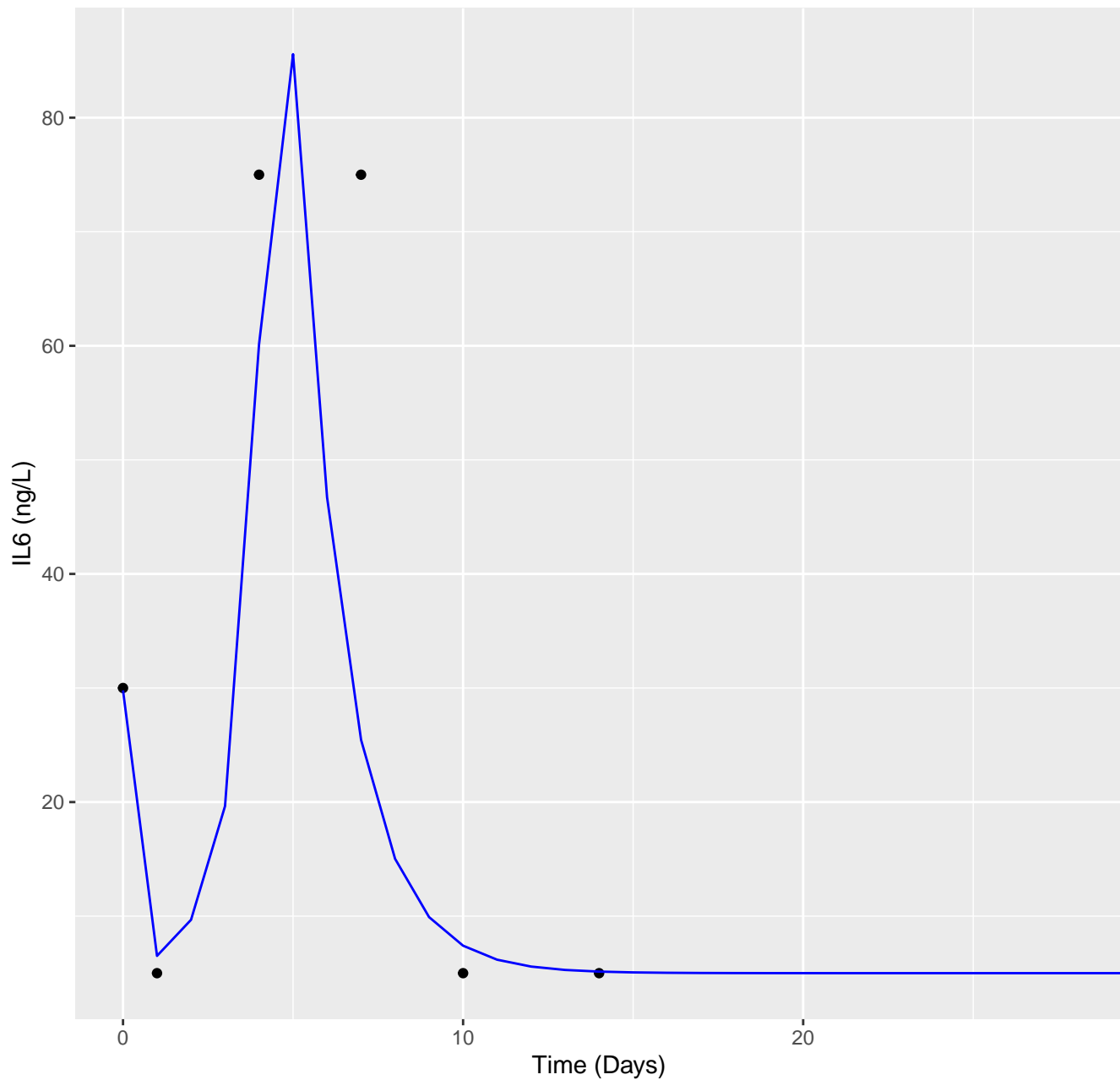
Model simulations IL6 for patient M57
