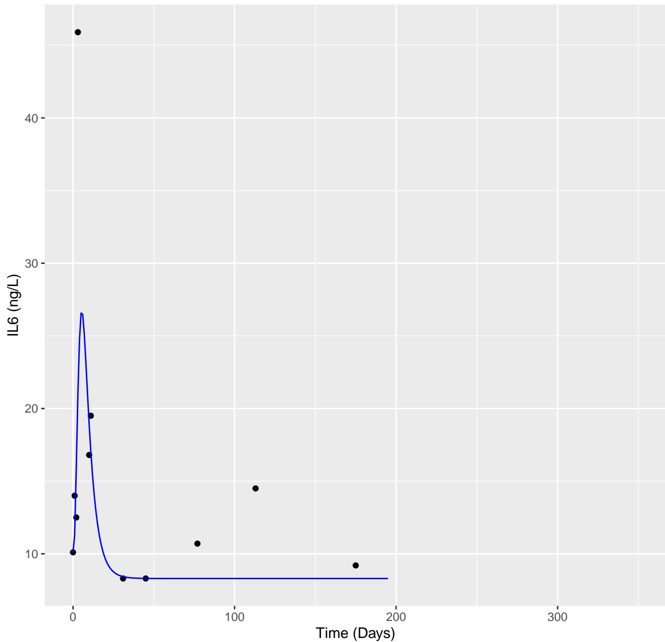
Model simulations IL6 for patient P03
