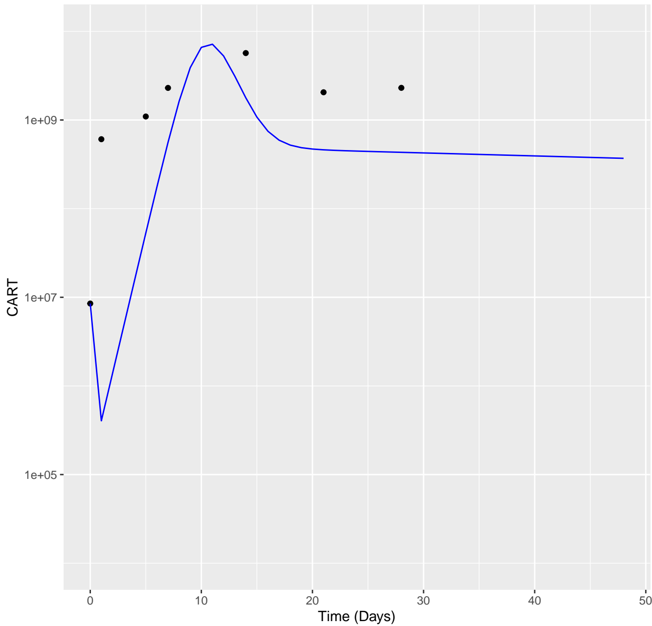
Model simulations CAR-T for patient M19
