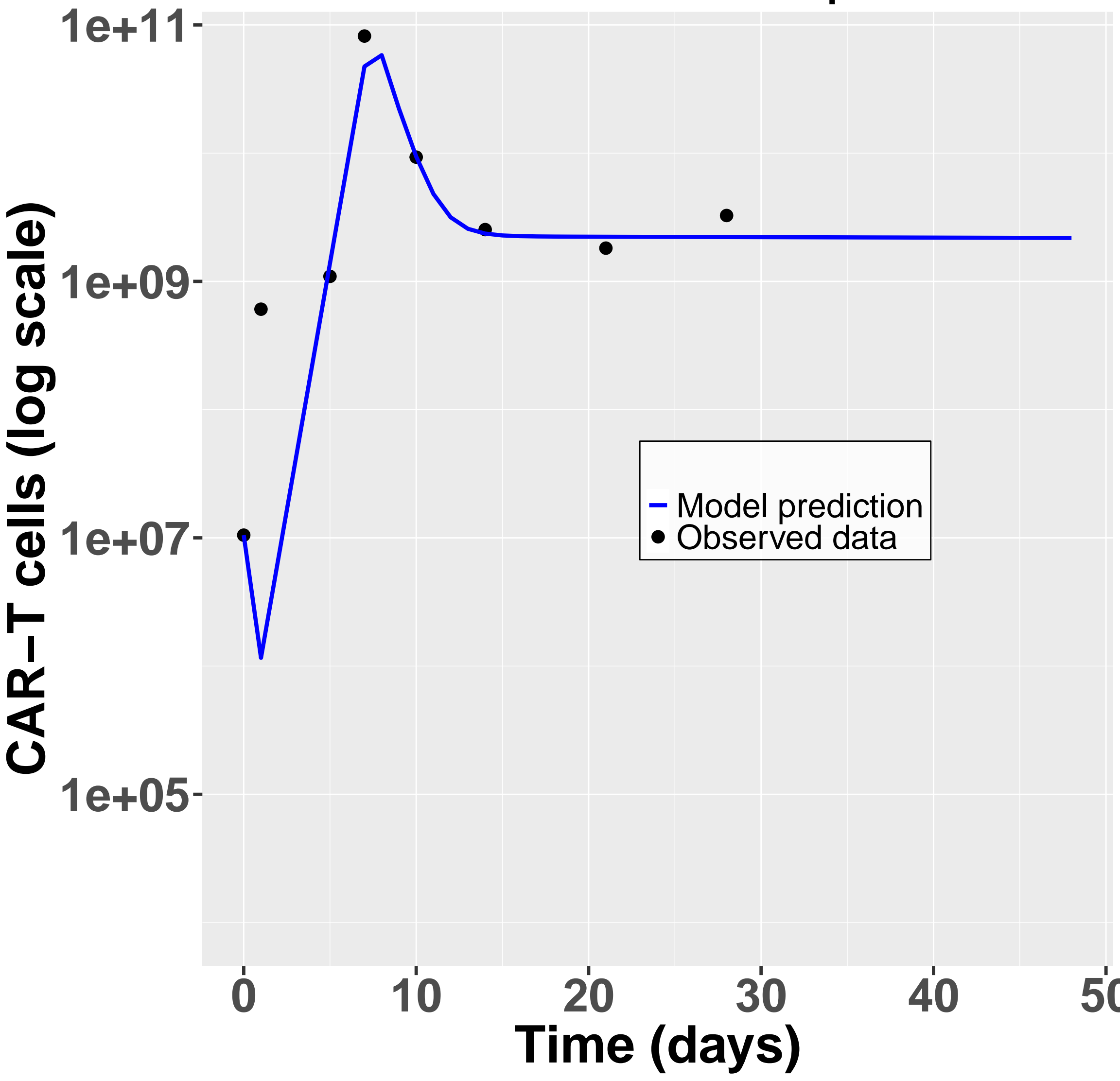
Model simulations CAR-T for patient M68
