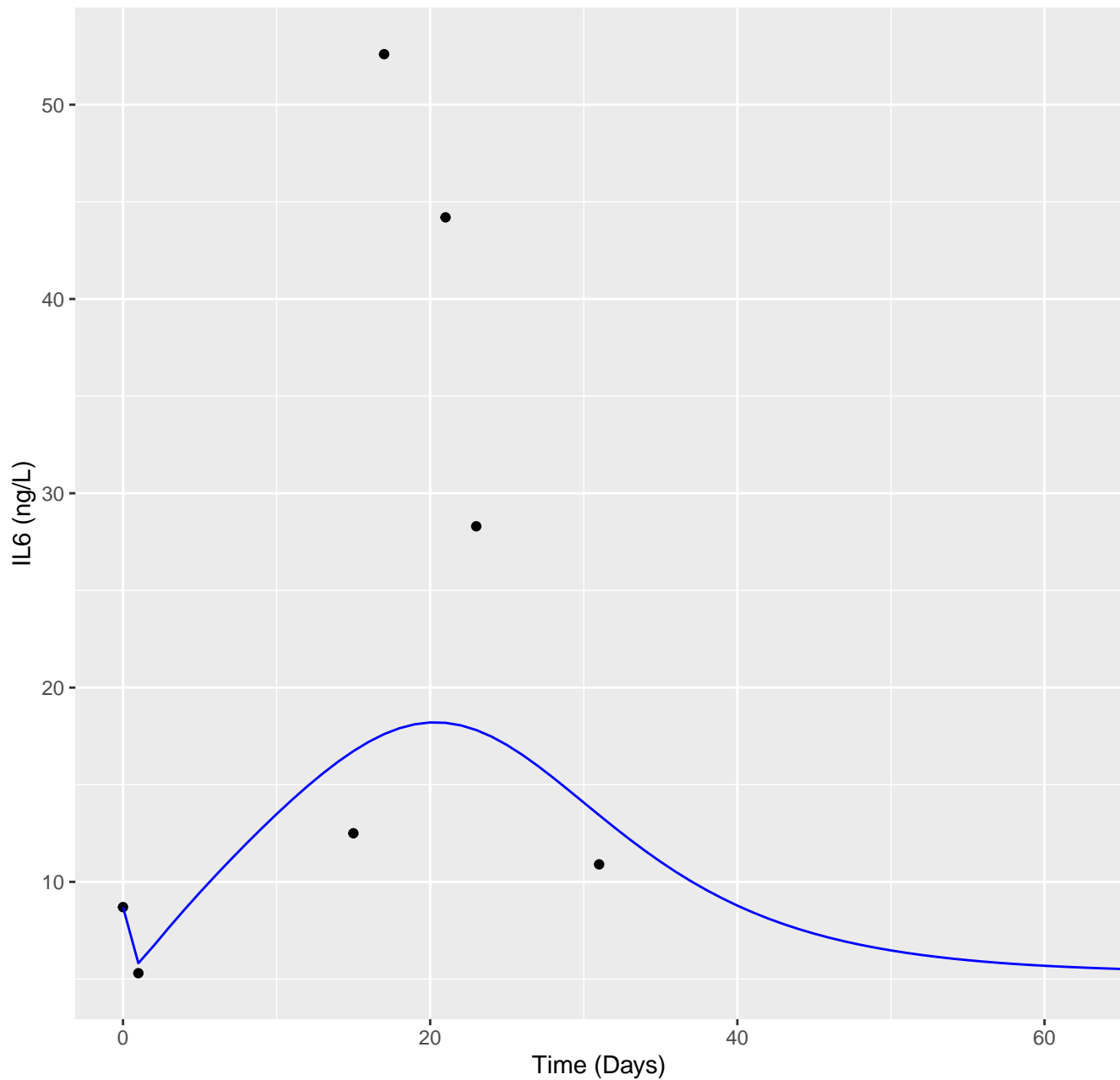
Model simulations IL6 for patient P02
