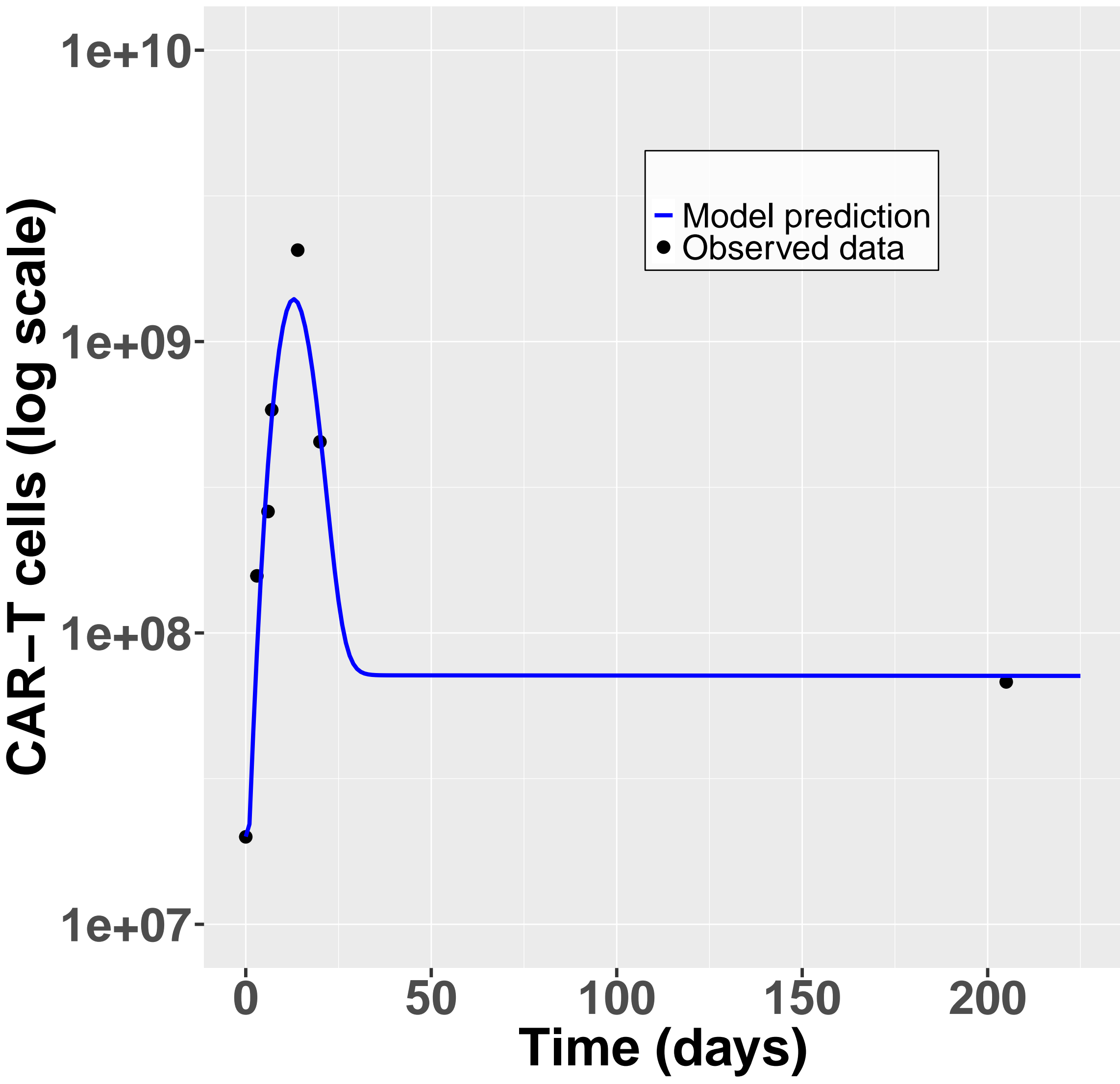
Model simulations CAR-T for patient L02
