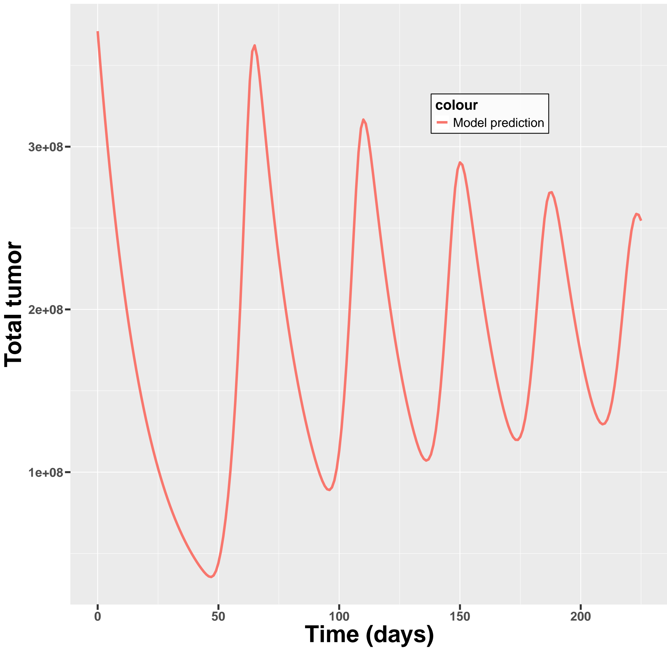
Model simulations of total tumor cells for patient L02
