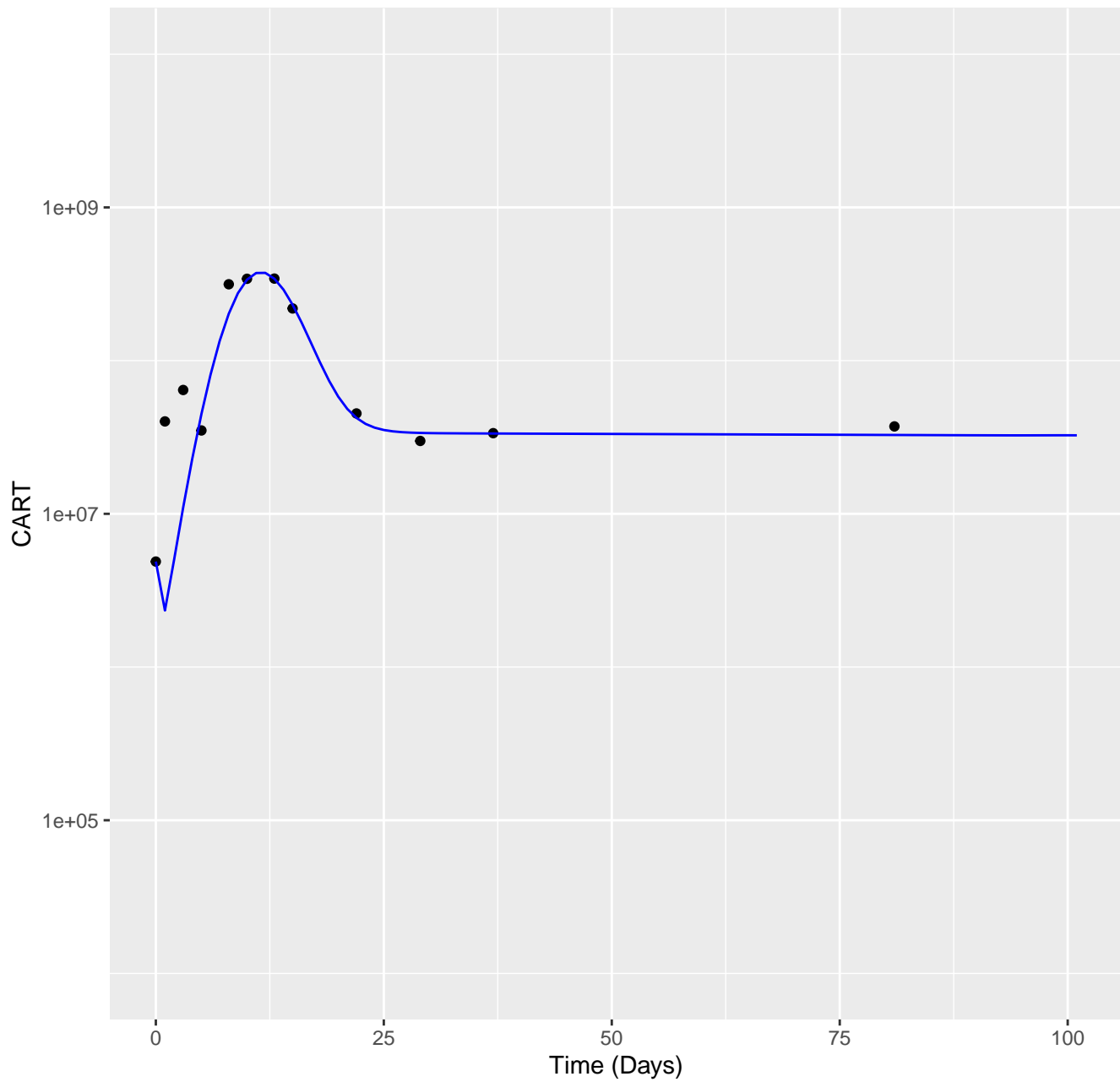
Model simulations CAR-T for patient L04
