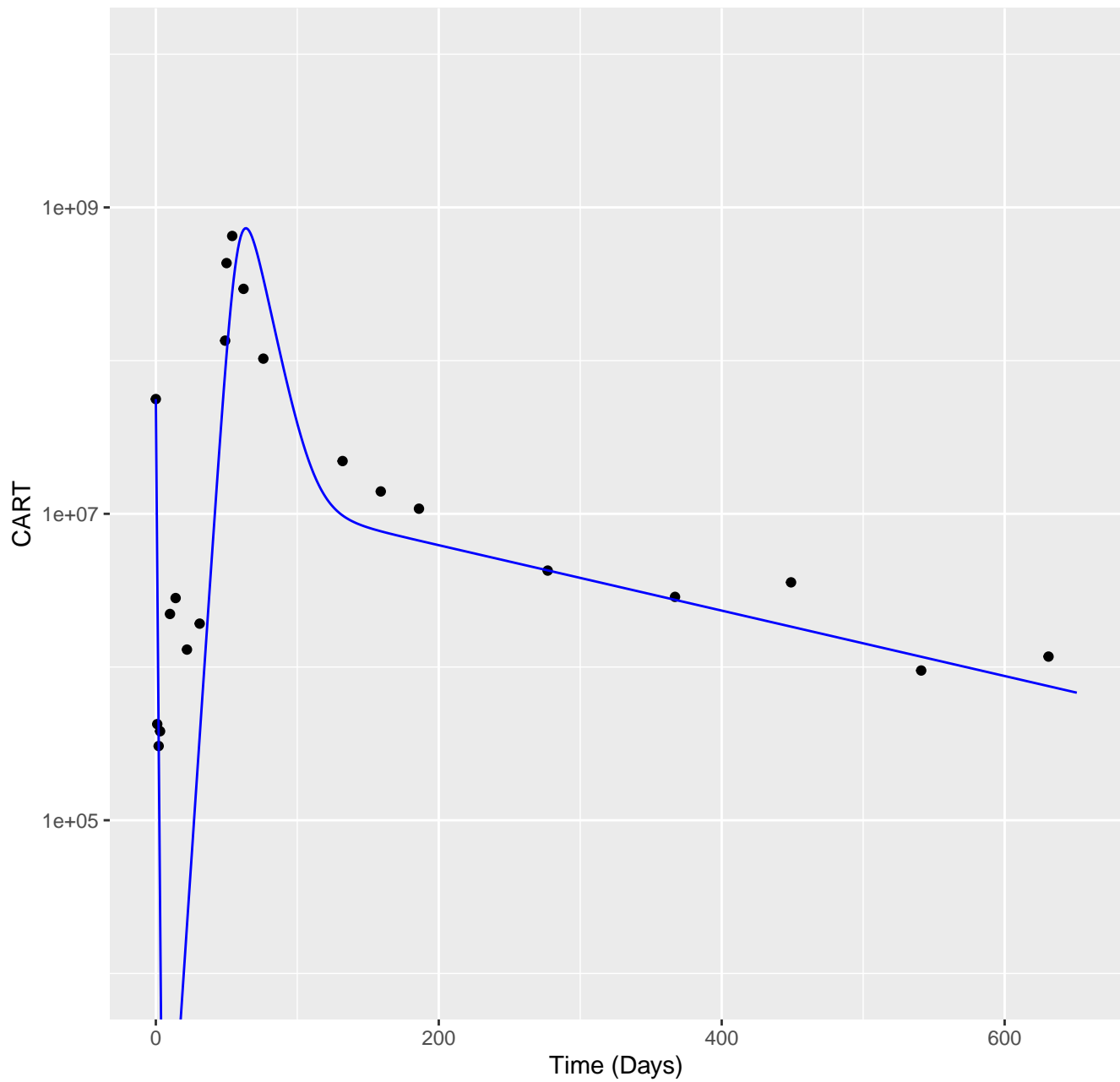
Model simulations CAR-T for patient P10
