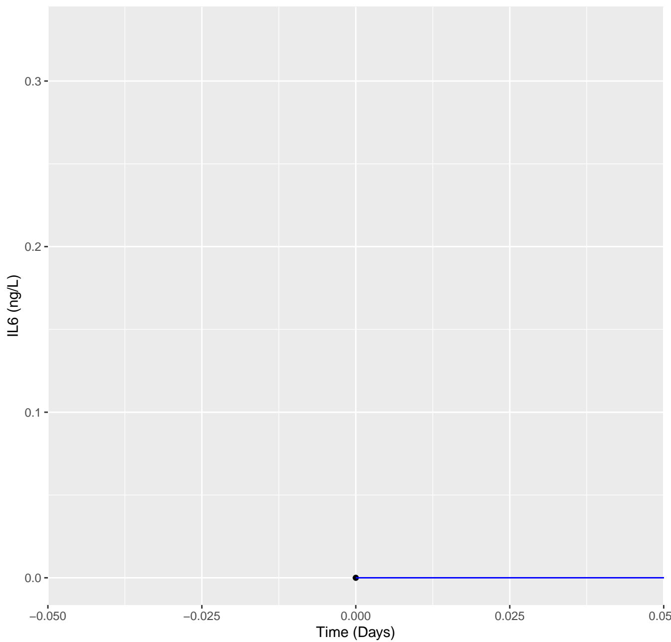
Model simulations IL6 for patient P22
