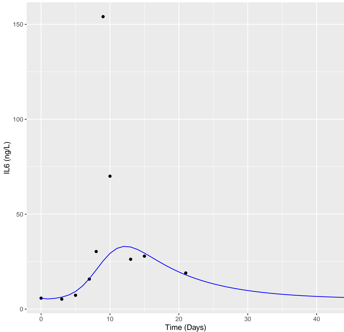
Model simulations IL6 for patient L04
