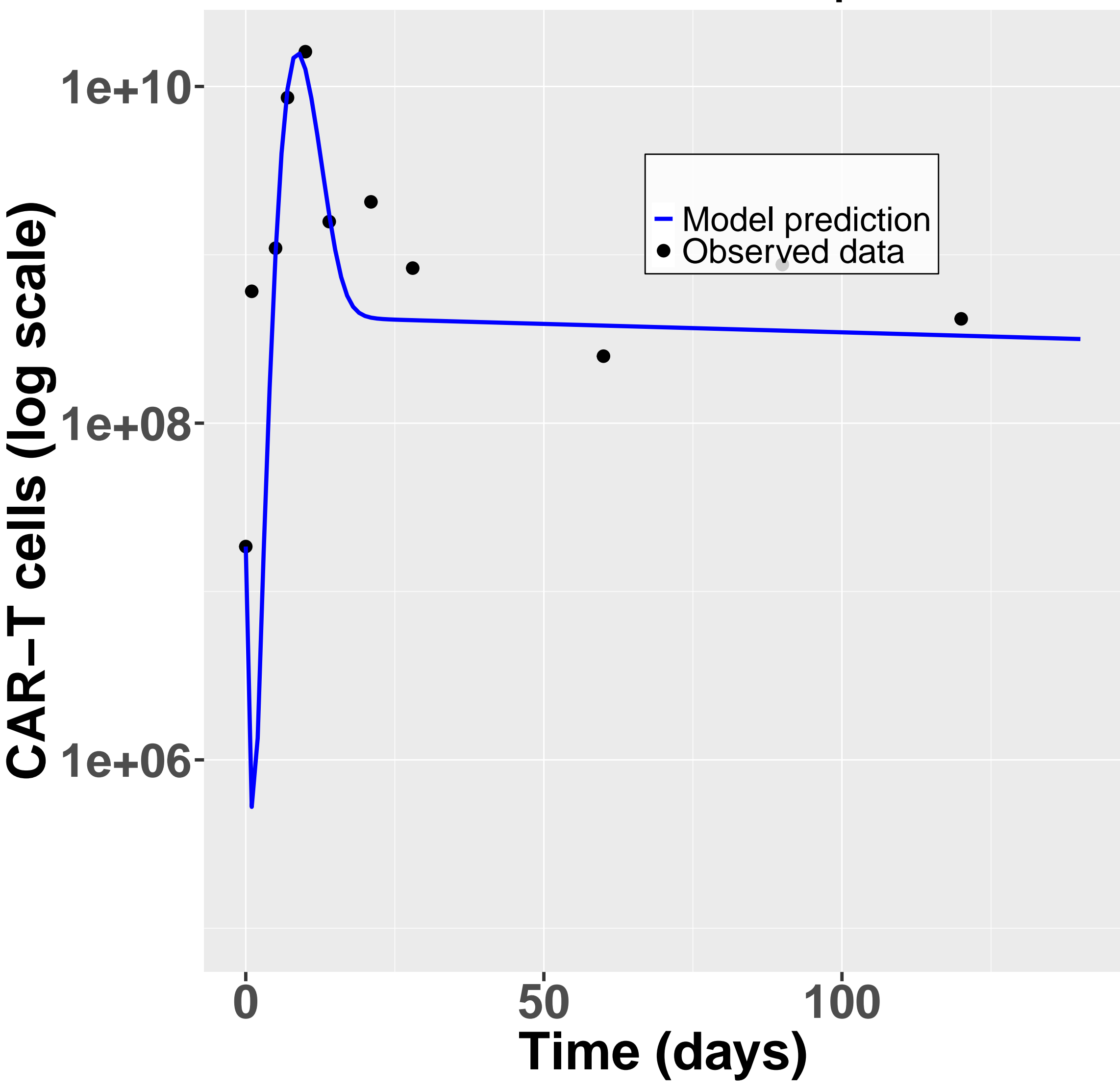
Model simulations CAR-T for patient M44
