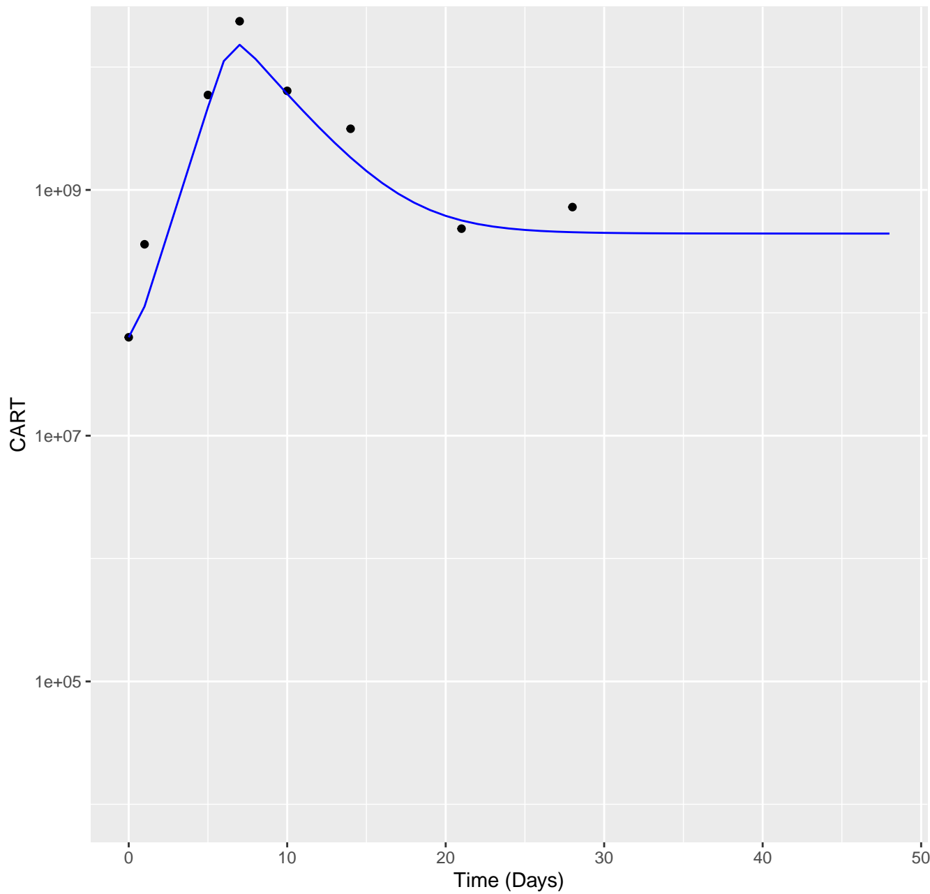
Model simulations CAR-T for patient M03
