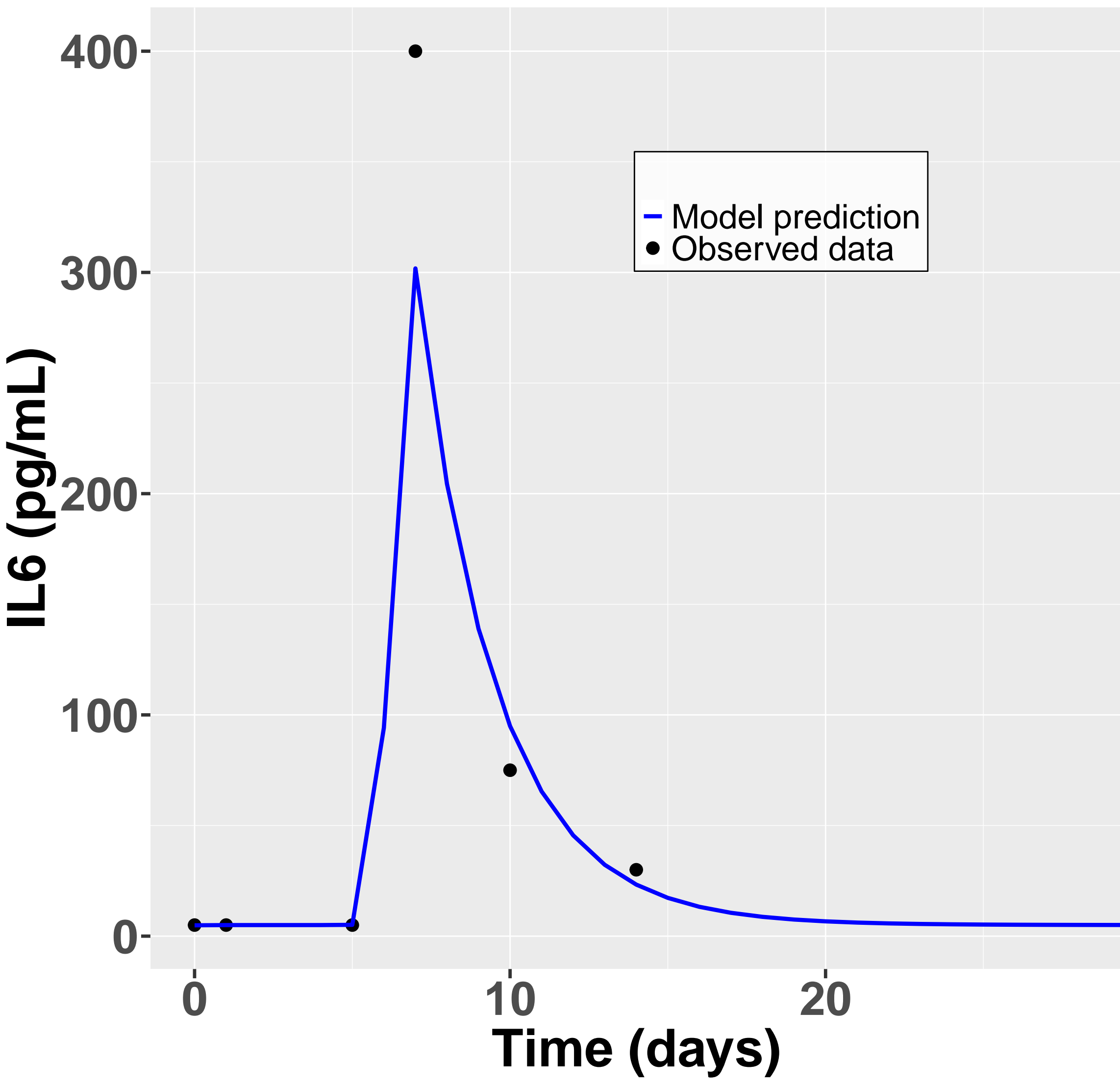
Model simulations of IL6 for patient M44
