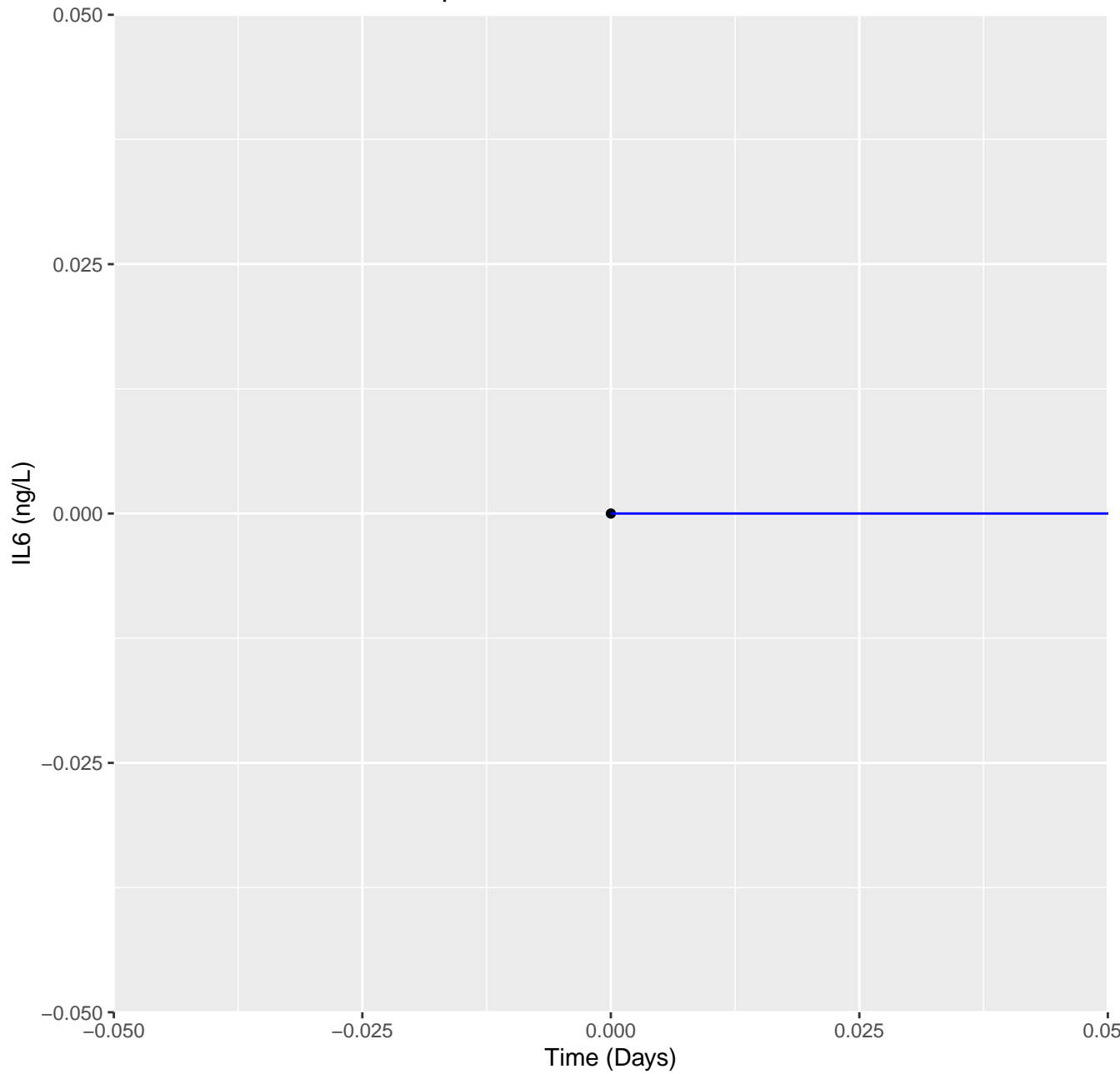
Model simulations IL6 for patient M09
