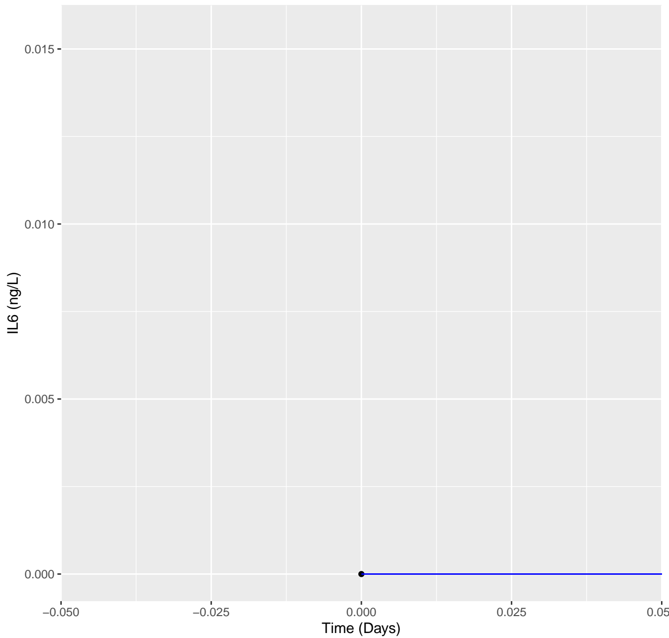
Model simulations IL6 for patient P12
