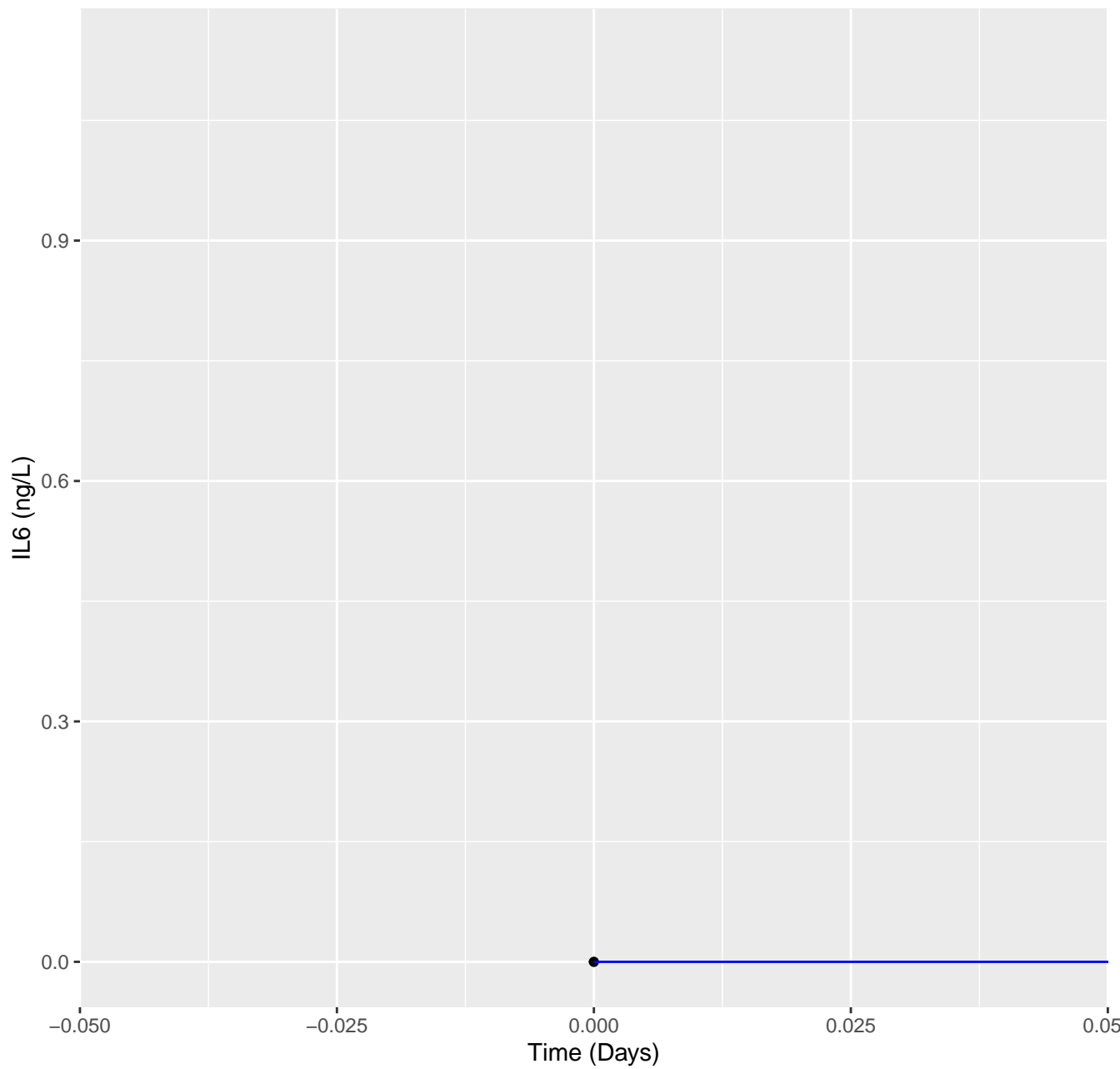
Model simulations IL6 for patient M19
