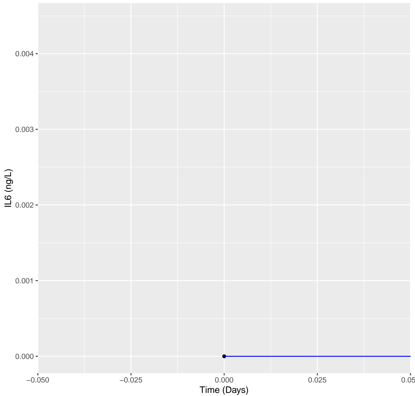
Model simulations IL6 for patient P05
