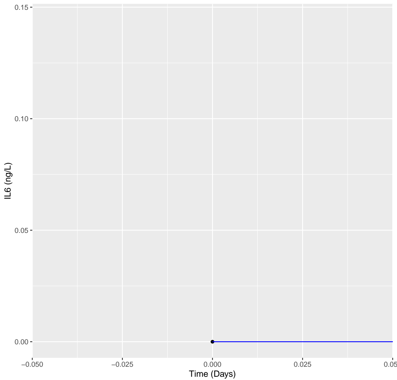
Model simulations IL6 for patient P10
