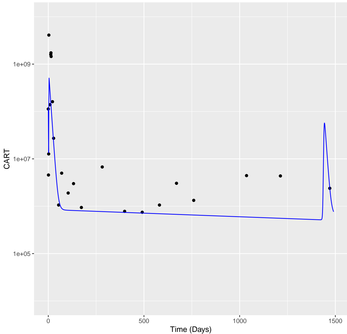
Model simulations CAR-T for patient P01
