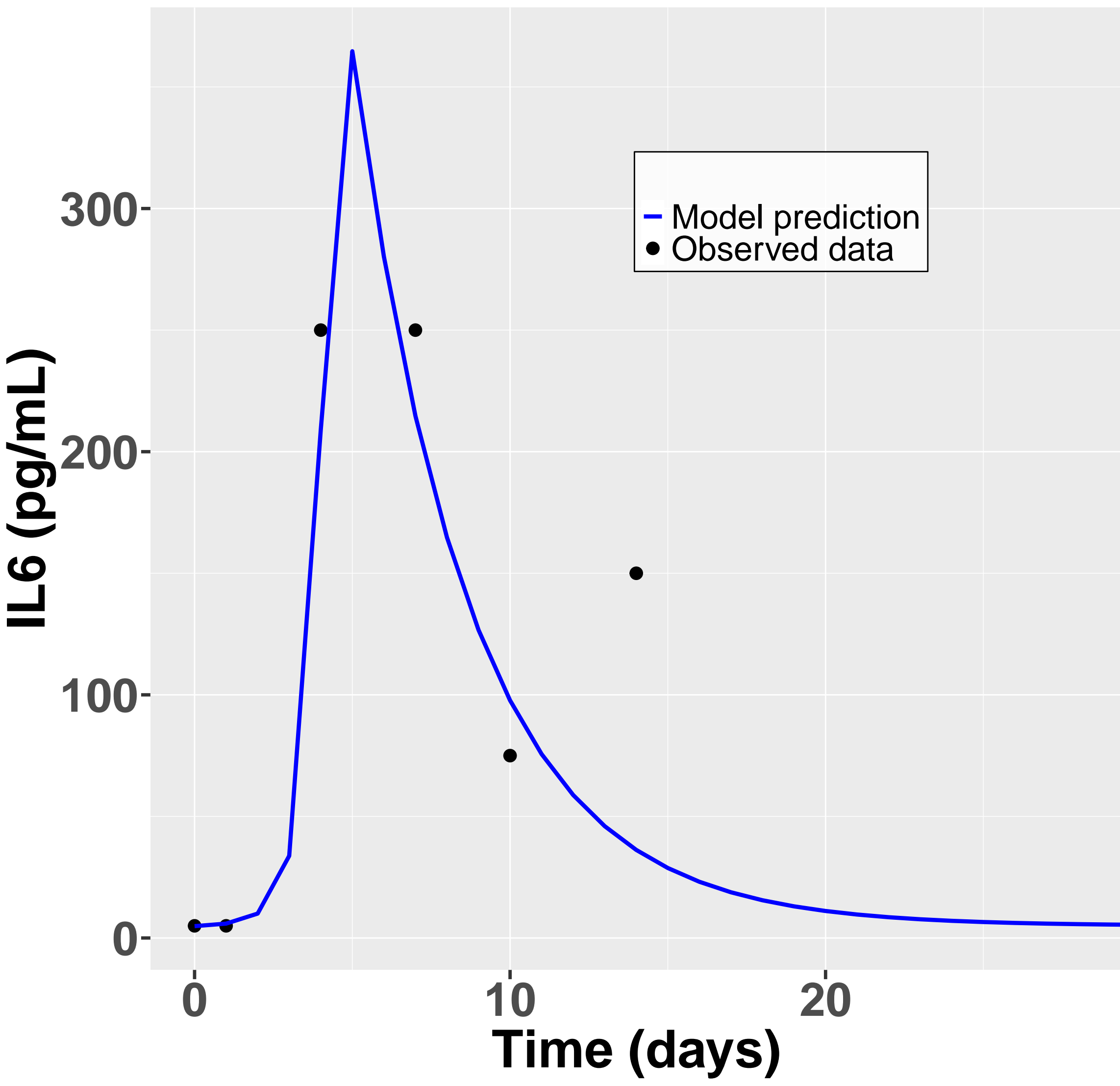
Model simulations of IL6 for patient M68
