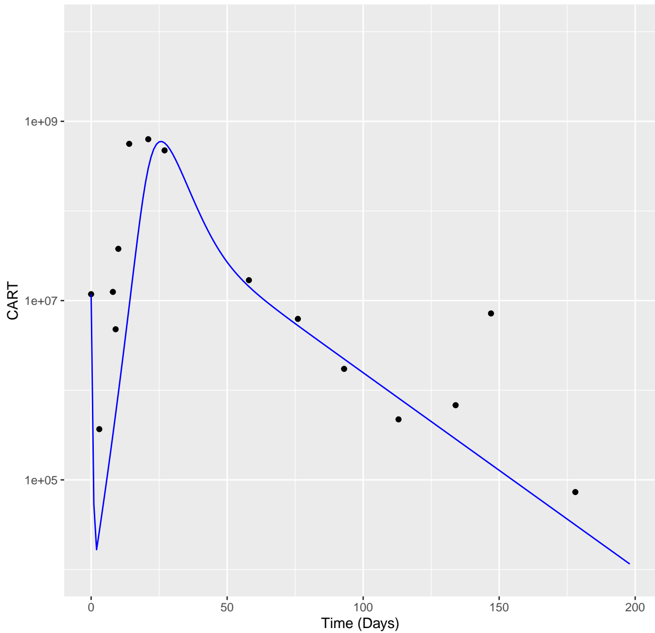
Model simulations CAR-T for patient P12
