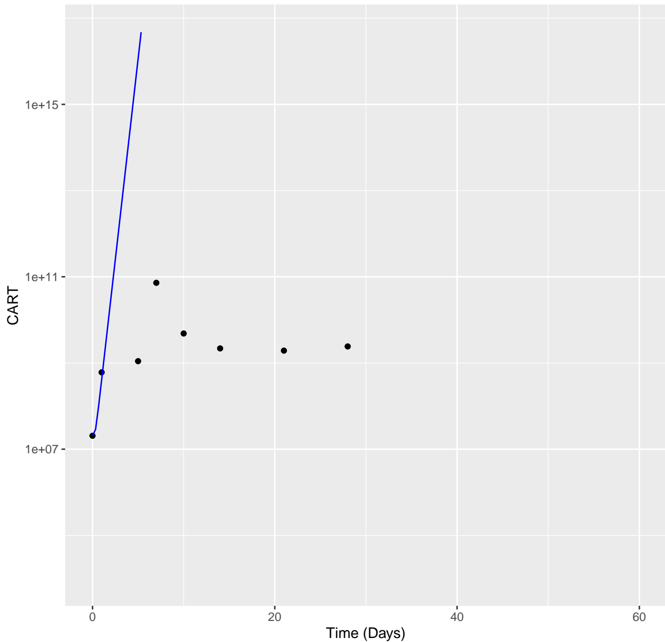
Model simulations CAR-T for patient M09
