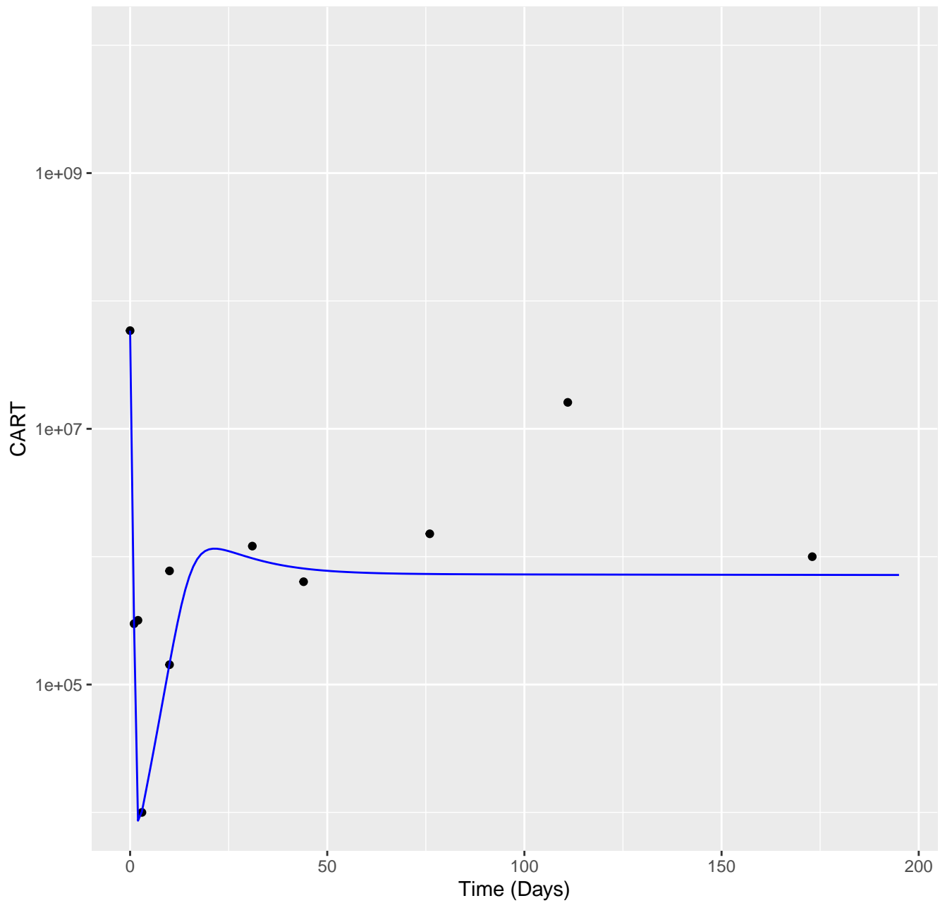
Model simulations CAR-T for patient P03
