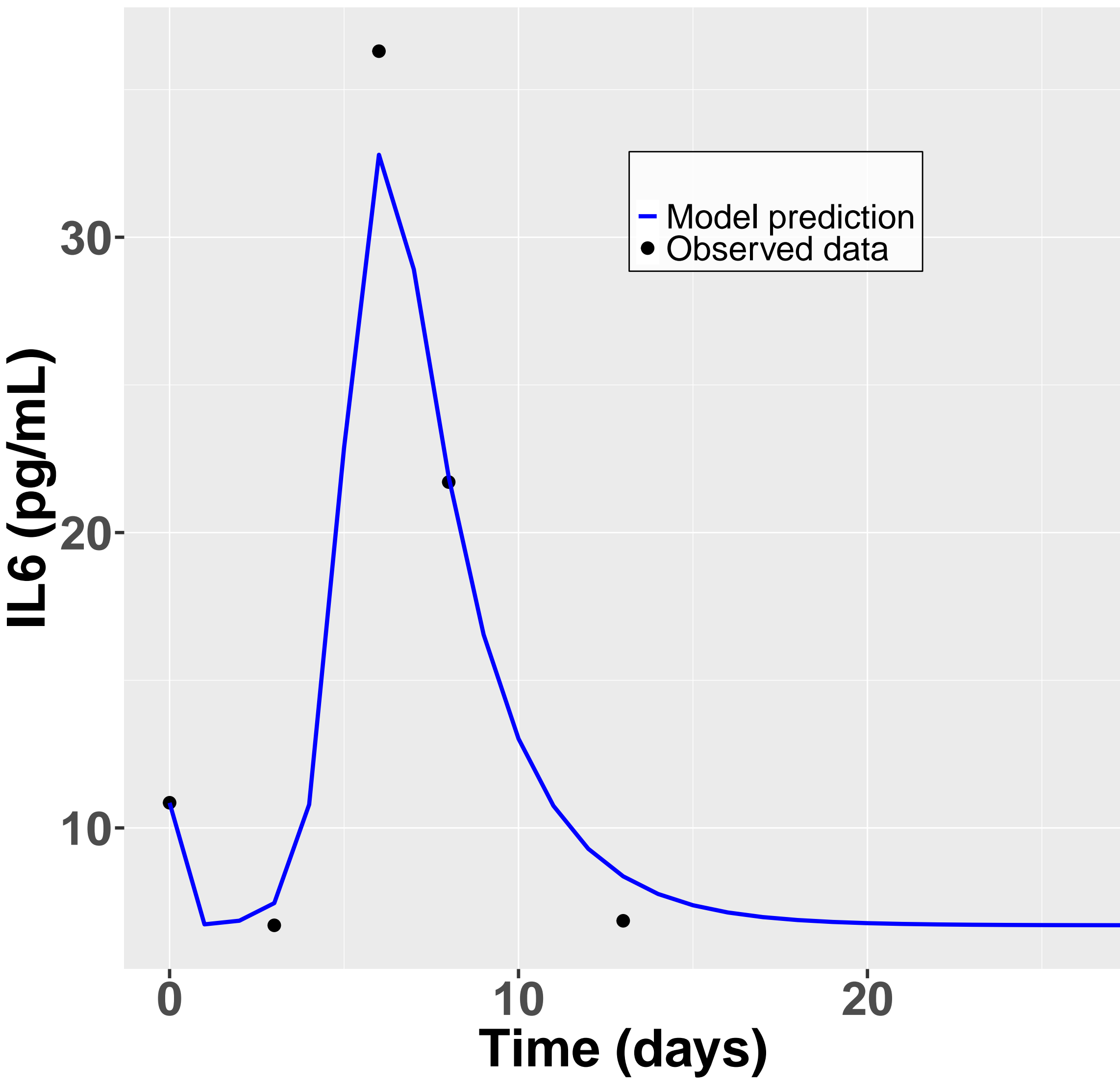
Model simulations of IL6 for patient L02
