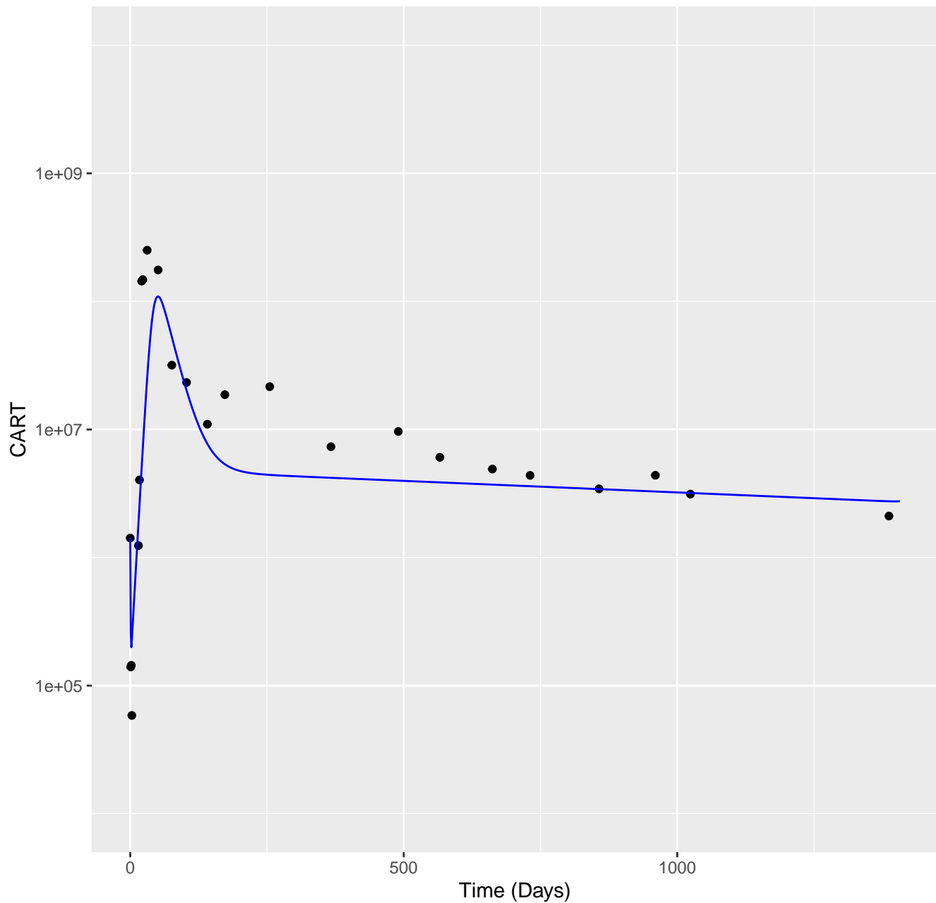
Model simulations CAR-T for patient P02
