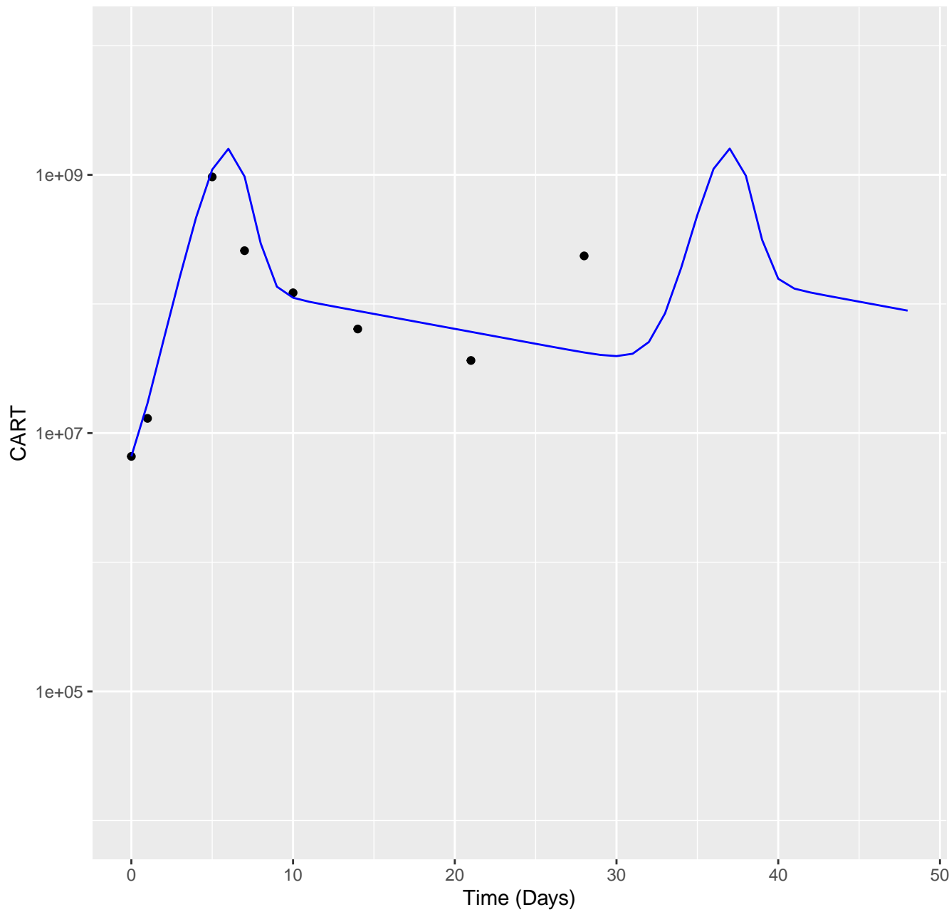
Model simulations CAR-T for patient M21
