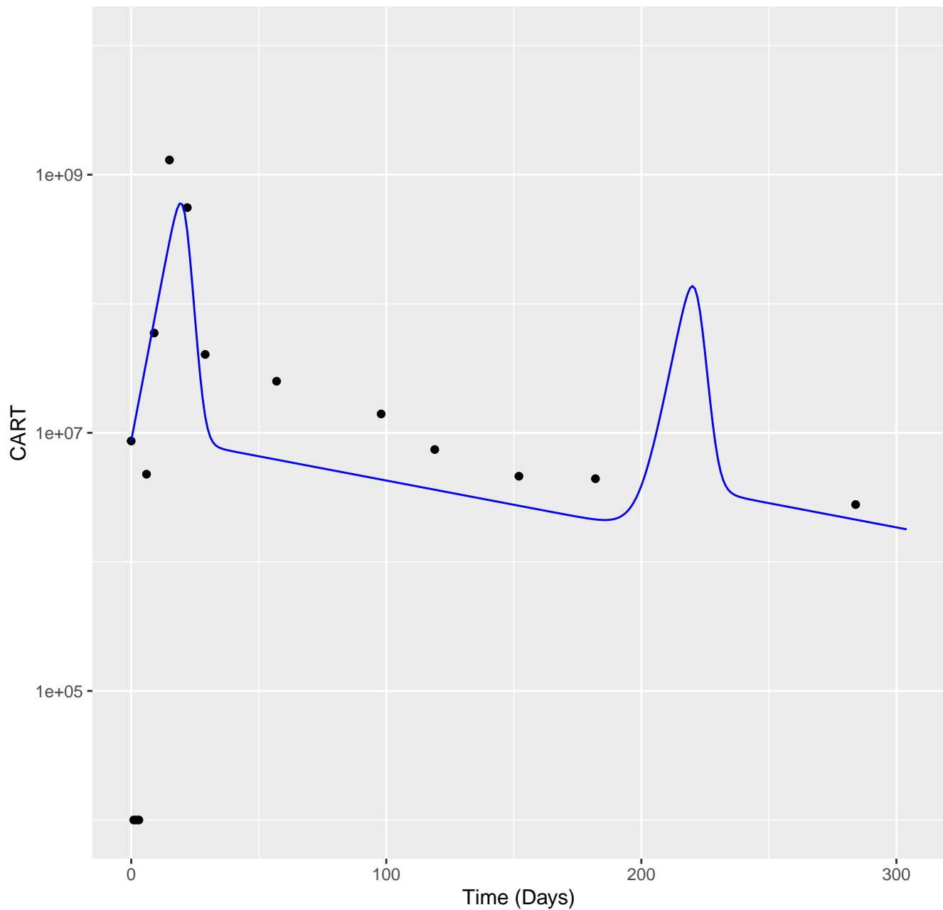
Model simulations CAR-T for patient P22
