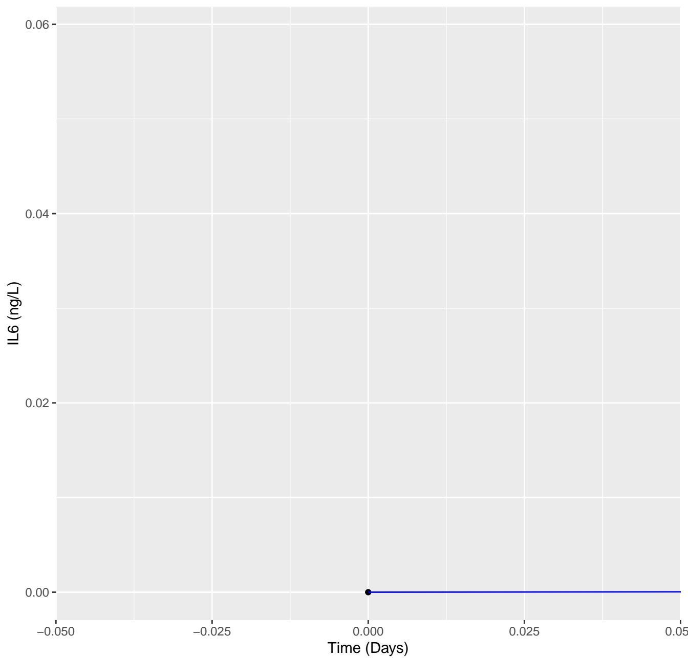
Model simulations IL6 for patient M21
