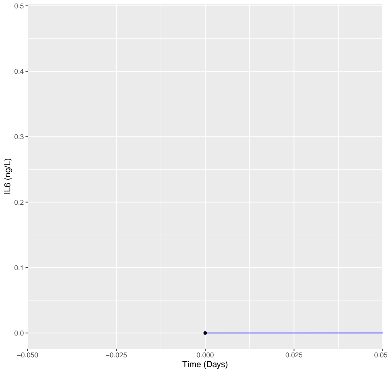
Model simulations IL6 for patient M03
