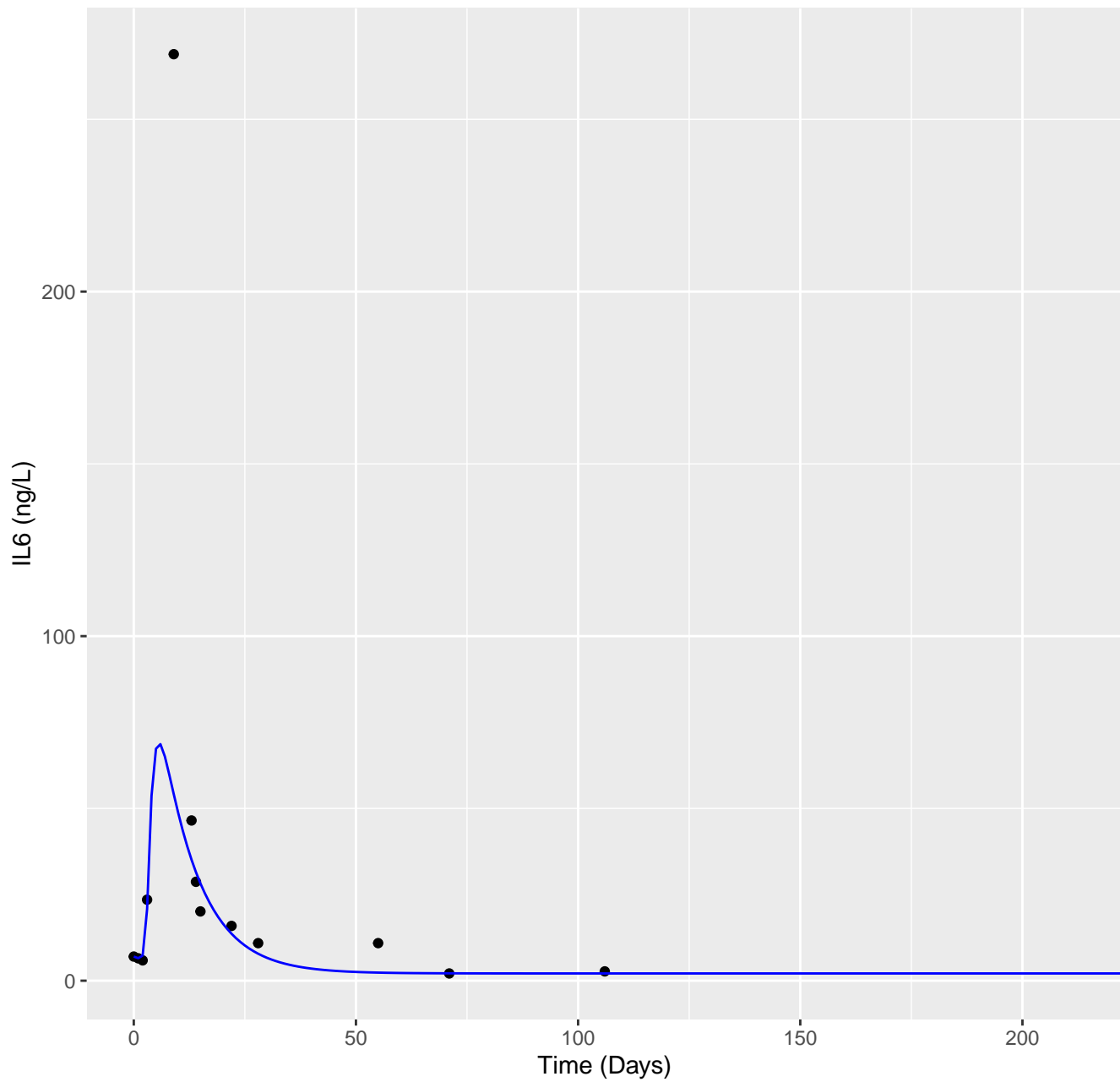
Model simulations IL6 for patient P01
