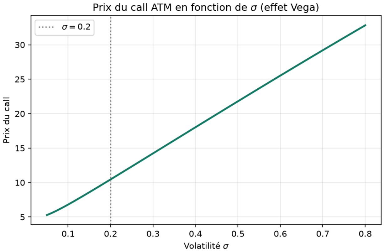
Figure 5: Figure 5 — Call vs \sigma
