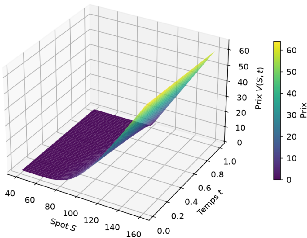
Figure 7: Figure 7 — Surface V(S, t)
