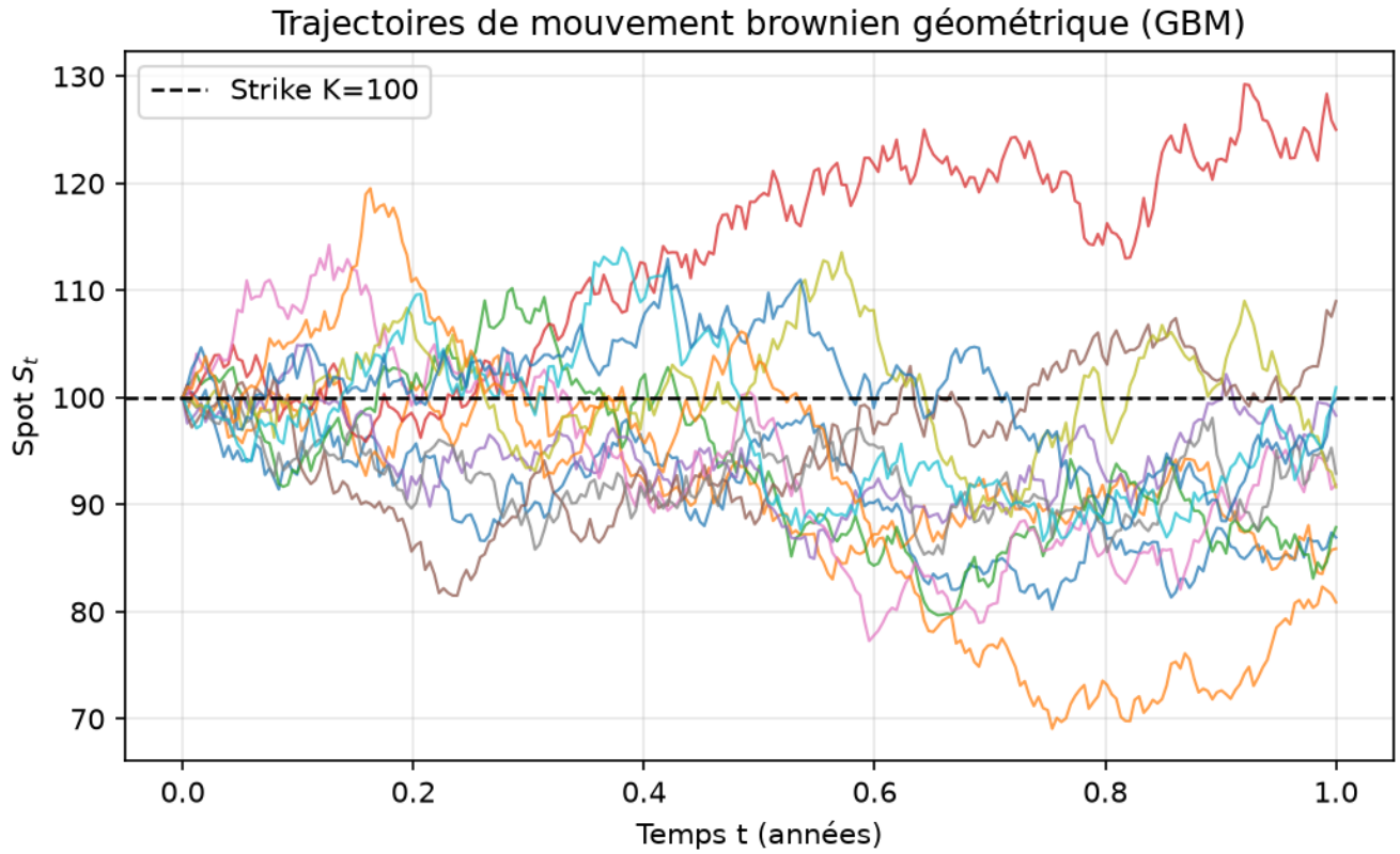
Figure 1: Figure 1 — Trajectoires GBM
