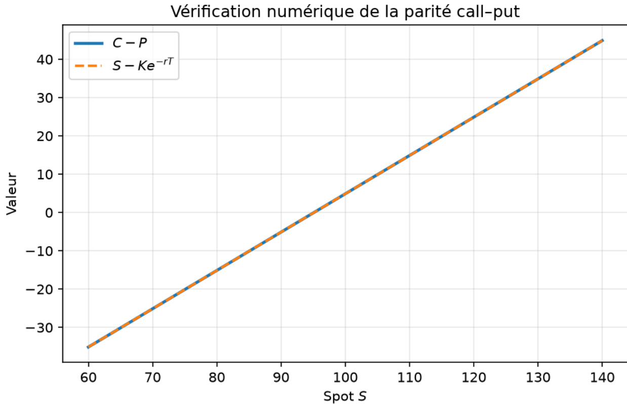
Figure 3: Figure 3 — Parité call-put
