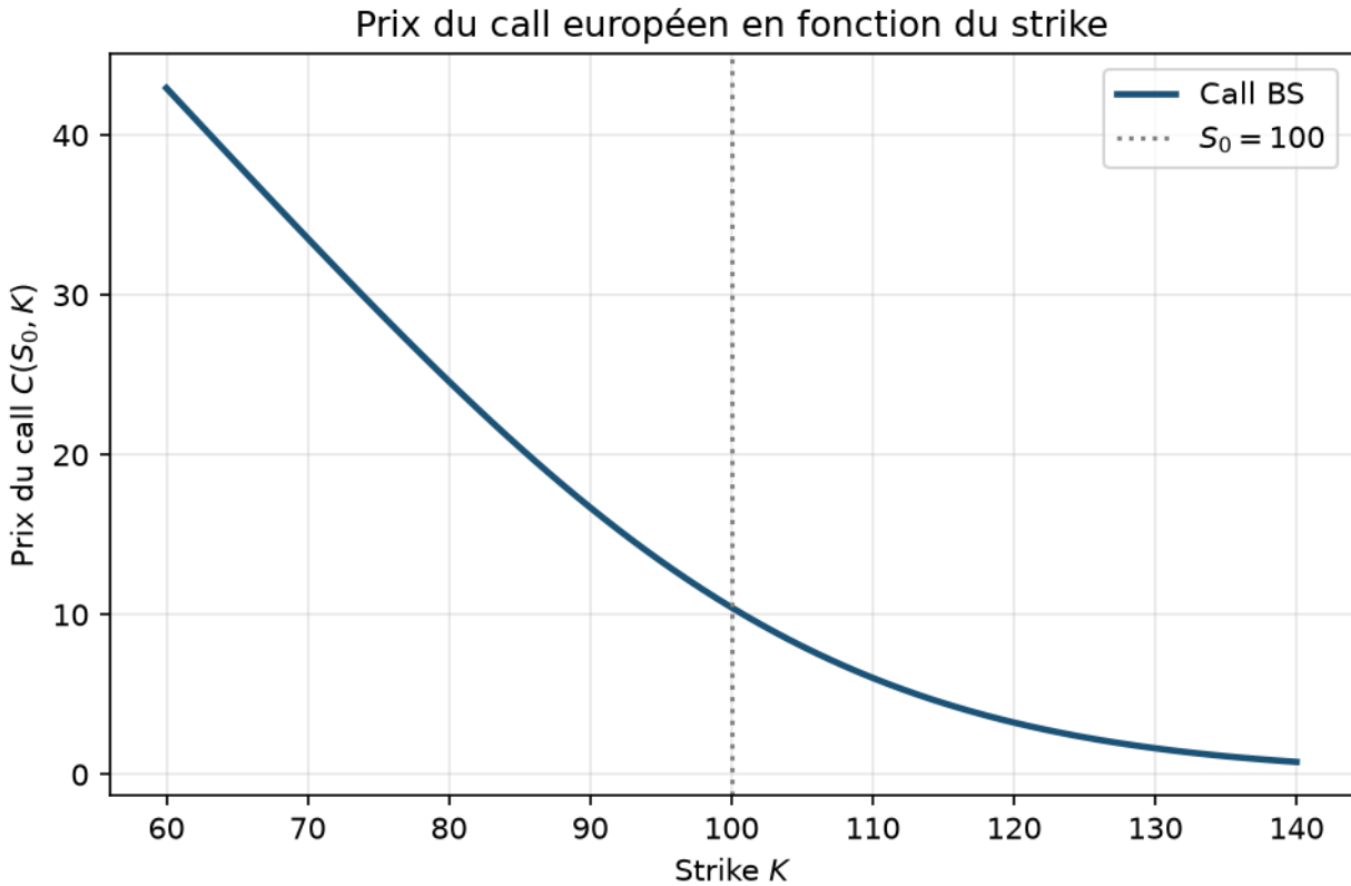
Figure 4: Figure 4 — Call vs K
