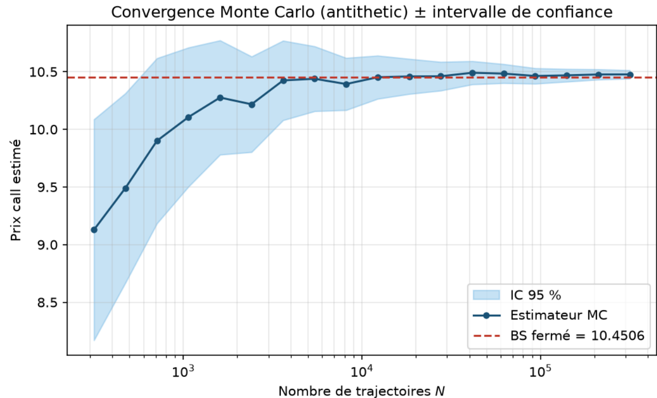
Figure 8: Figure 8 — Convergence MC
