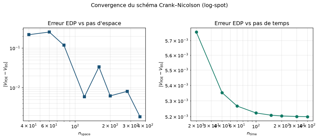
Figure 9: Figure 9 — Erreurs EDP
