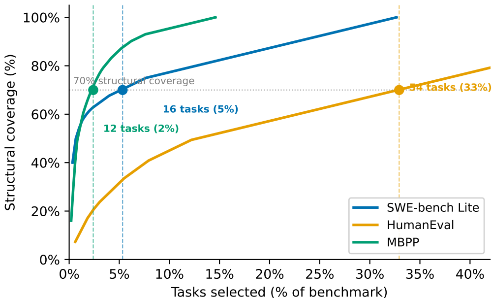
Structural saturation across benchmarks (greedy set cover, AST-edit distance, t = 0.28 )
