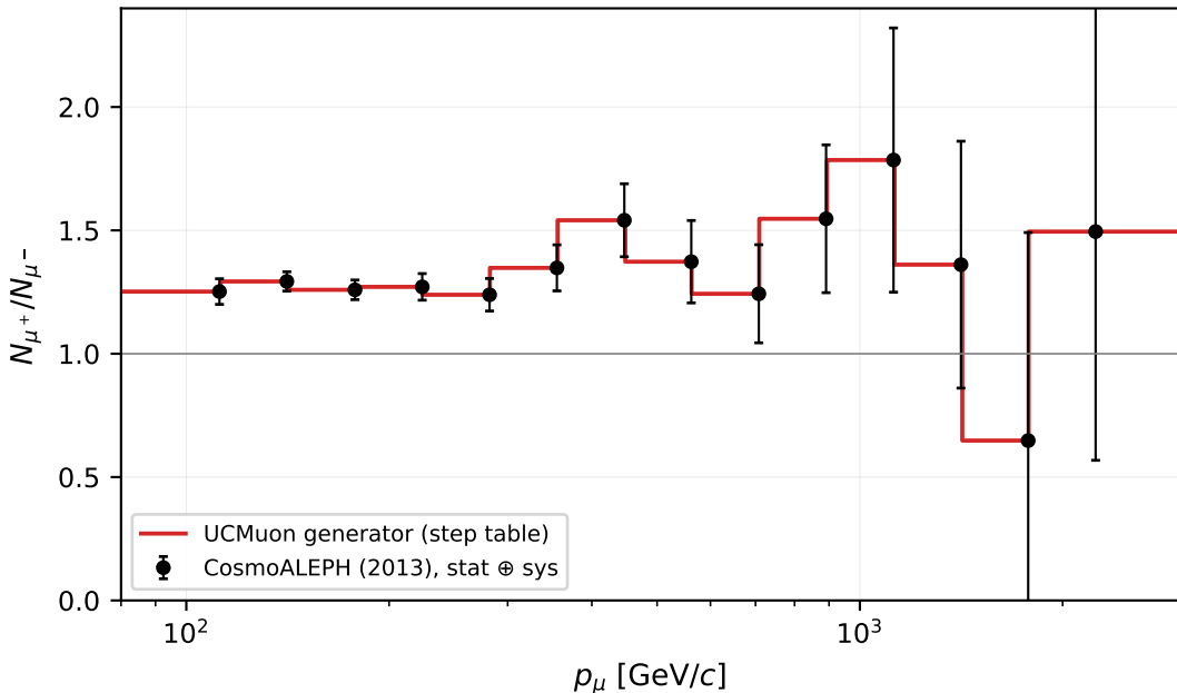
Muon charge ratio: generator table vs. CosmoALEPH
