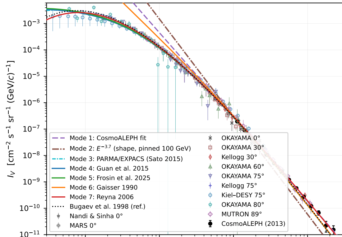
UCMuon source spectra vs. sea-level vertical muon data
