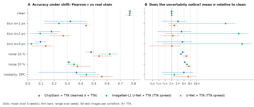
Figure 6. (A) Pearson r with the real stain under each shift. (B) Mean \sigma relative to the clean image (log scale). ChipStain (blue) and the U-Net (orange) both use 8x TTA; the U-Net's \sigma is its TTA disagreement.
