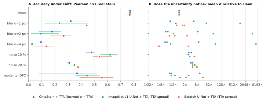
Figure 6. (A) Pearson r with the real stain under each shift. (B) Mean \sigma relative to the clean image (log scale). Dots are means over three seeds and thin bars the range over seeds; a mean above 1\times can hide seeds in which \sigma falls (Table 7b). All models use 8\times TTA; for the L1 U-Nets \sigma is the TTA disagreement.
