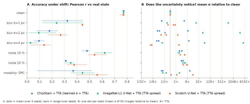
Figure 6. (A) Pearson r with the real stain under each shift. (B) Mean \sigma relative to the clean image (log scale). Dots are means over three seeds and thin bars the range over seeds; a mean above 1\times can hide seeds in which \sigma falls (Table 7b). All models use 8\times TTA; for the L1 U-Nets \sigma is the TTA disagreement.
