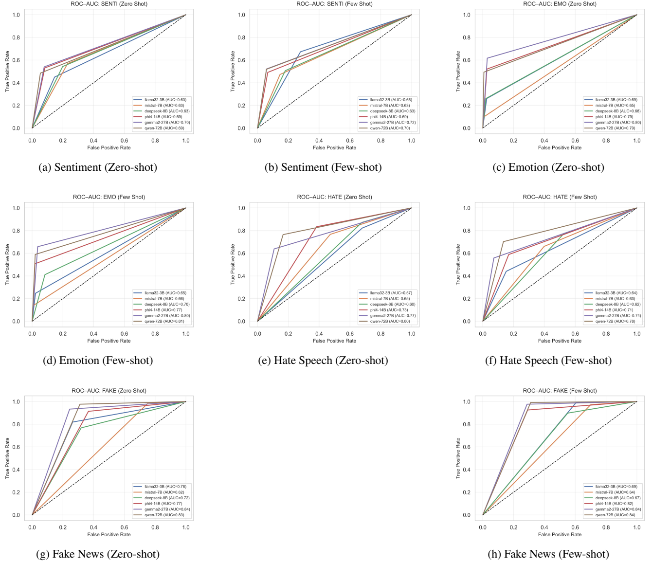
FIGURE 17: ROC-AUC curves of six LLMs on Bengali text classification tasks under zero- and few-shot settings.
