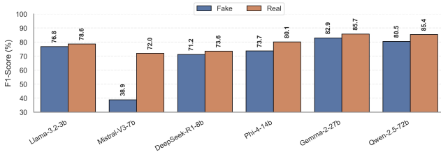
(a) Zero-shot setting
