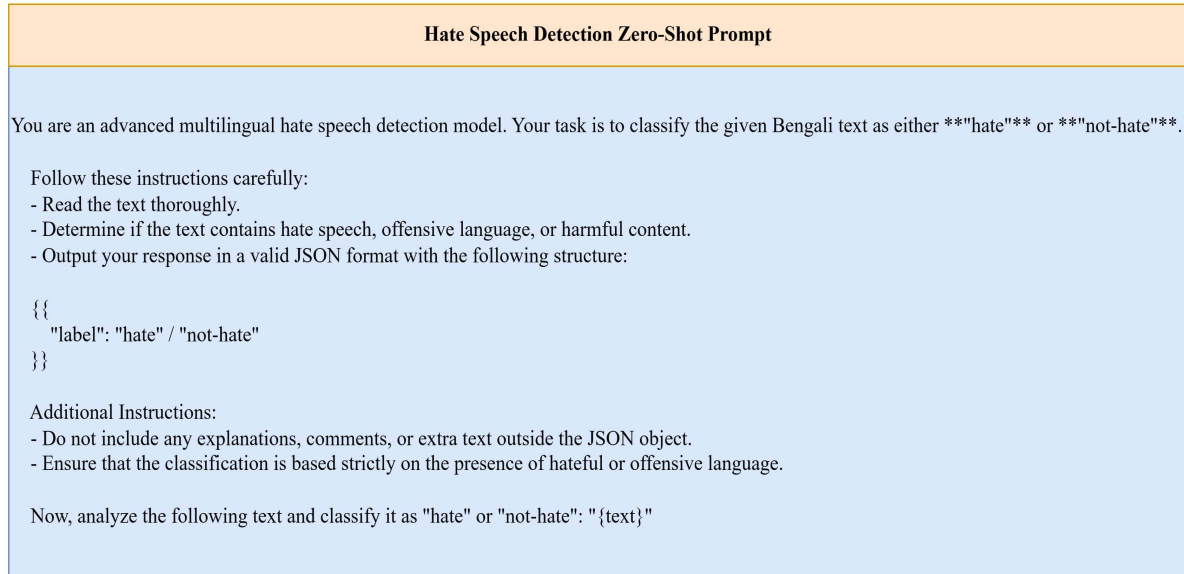
FIGURE 5: Prompt used for zero-shot Bengali Hate Speech Detection.
