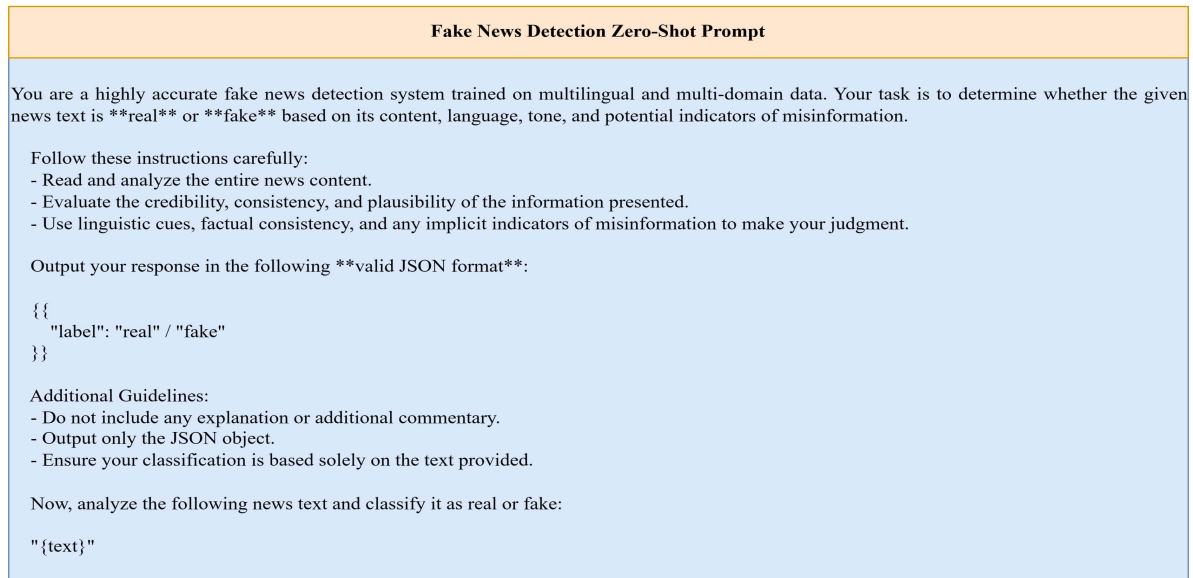
FIGURE 6: Prompt used for zero-shot Bengali Fake News Detection.
