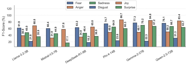
(a) Zero-shot setting
