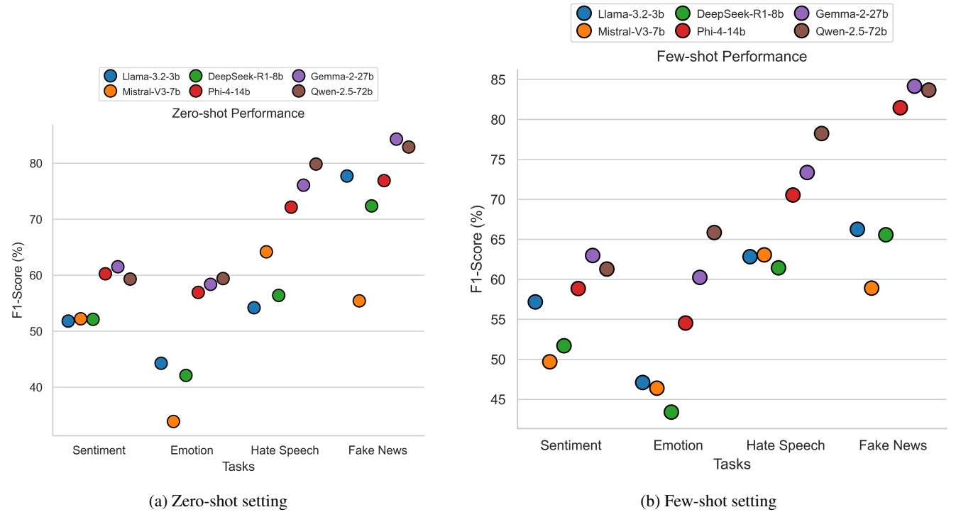
FIGURE 18: LLMs' performance with two prompt settings across various classification tasks.
