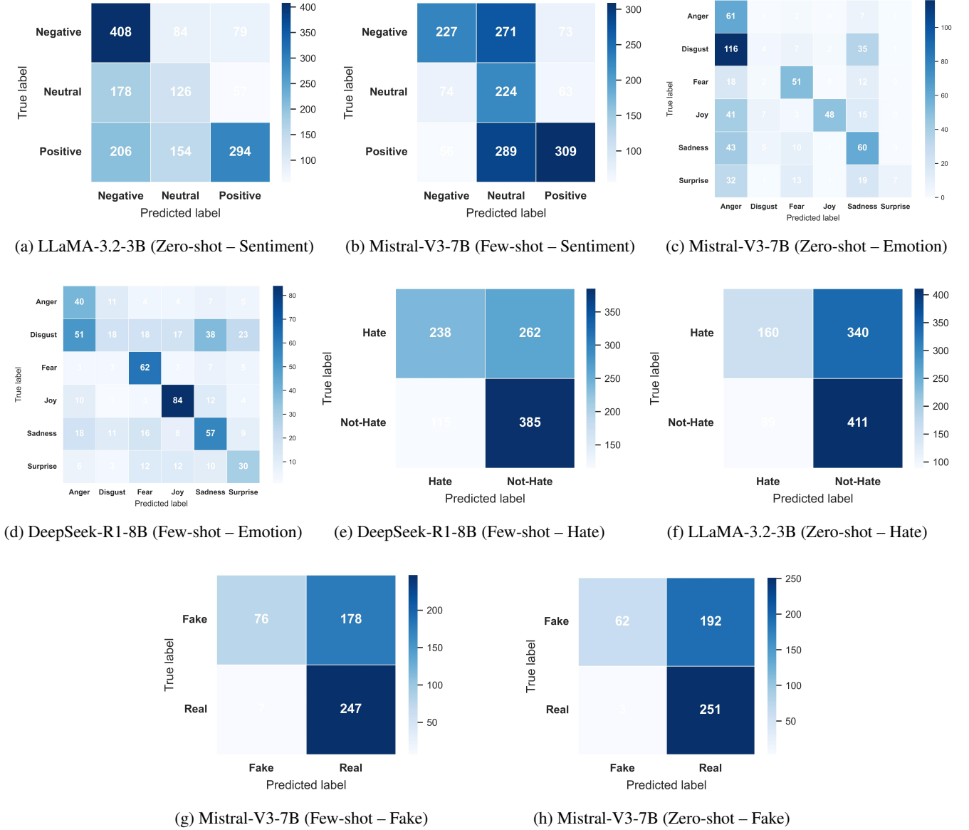
FIGURE 16: Confusion matrices of low-performing LLMs showing misclassification patterns in Bengali tasks.
