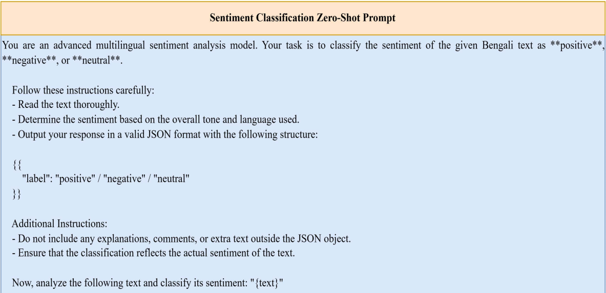
FIGURE 3: Prompt used for zero-shot Bengali Sentiment Analysis.
