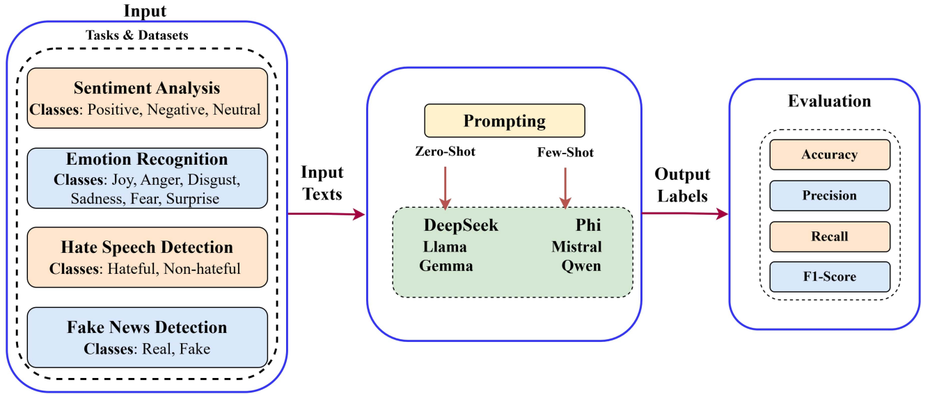
FIGURE 2: Overall methodology illustrating the evaluation framework for six open-source LLMs across four Bengali text classification tasks under zero-shot and few-shot prompting
