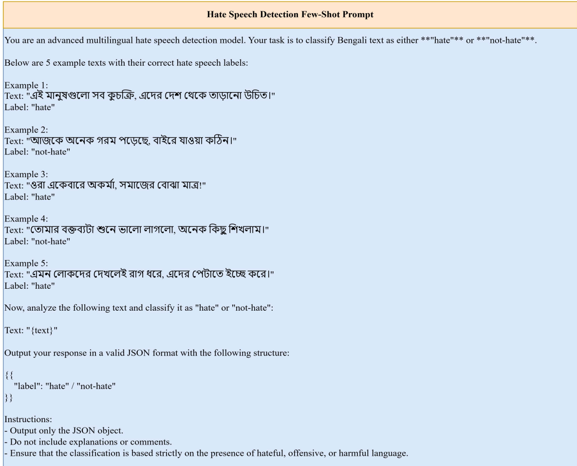
FIGURE 9: Prompt used for few-shot Bengali Hate Speech Detection.
