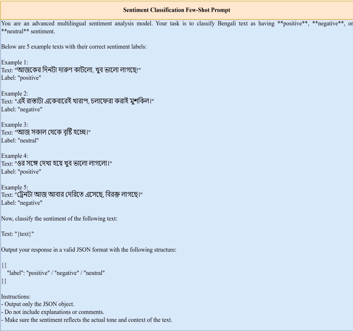
FIGURE 7: Prompt used for few-shot Bengali Sentiment Analysis.
