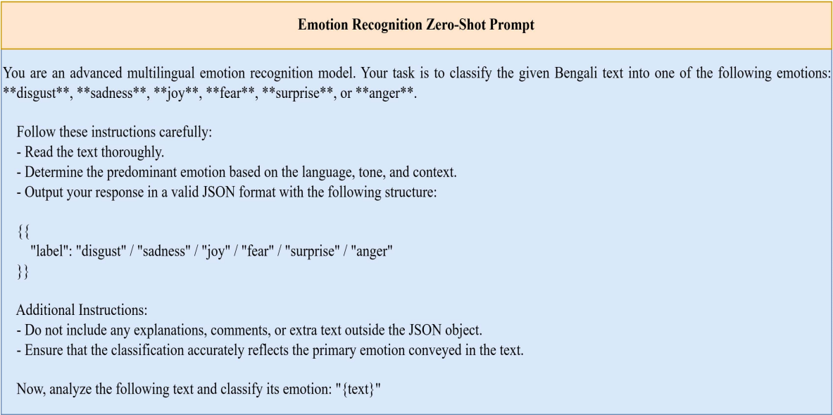
FIGURE 4: Prompt used for zero-shot Bengali Emotion Recognition.
