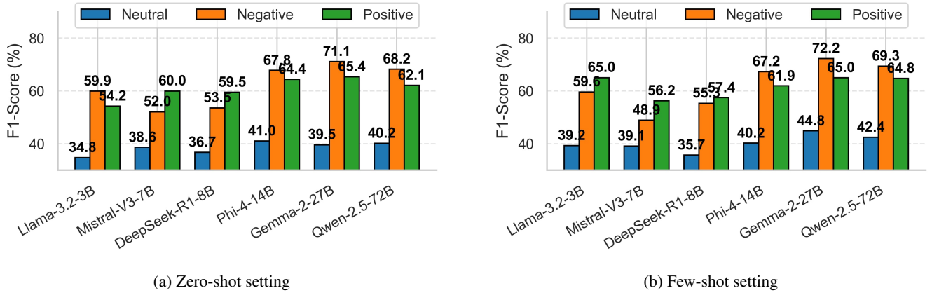
FIGURE 11: Class-wise sentiment classification performance for two prompt settings across LLMs.
