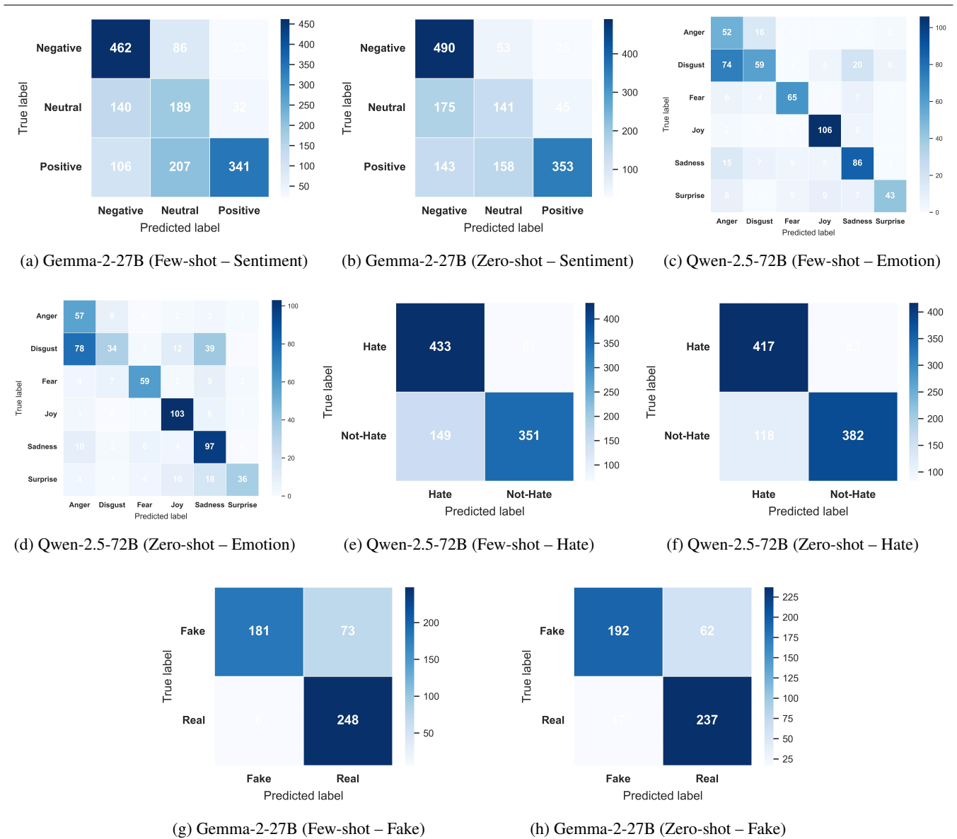
FIGURE 15: Confusion matrices of top LLMs on Bengali text classification tasks under zero- and few-shot settings.
