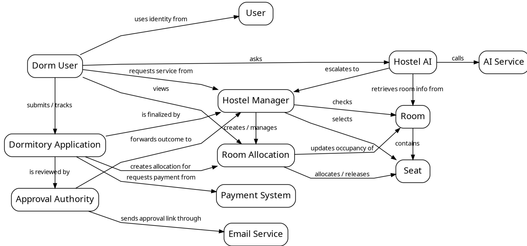
Fig CRC.4: Dormitory Module Collaboration Diagram
