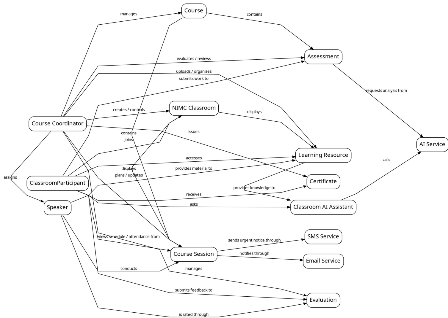
Fig CRC.2: Classroom Module Collaboration Diagram
