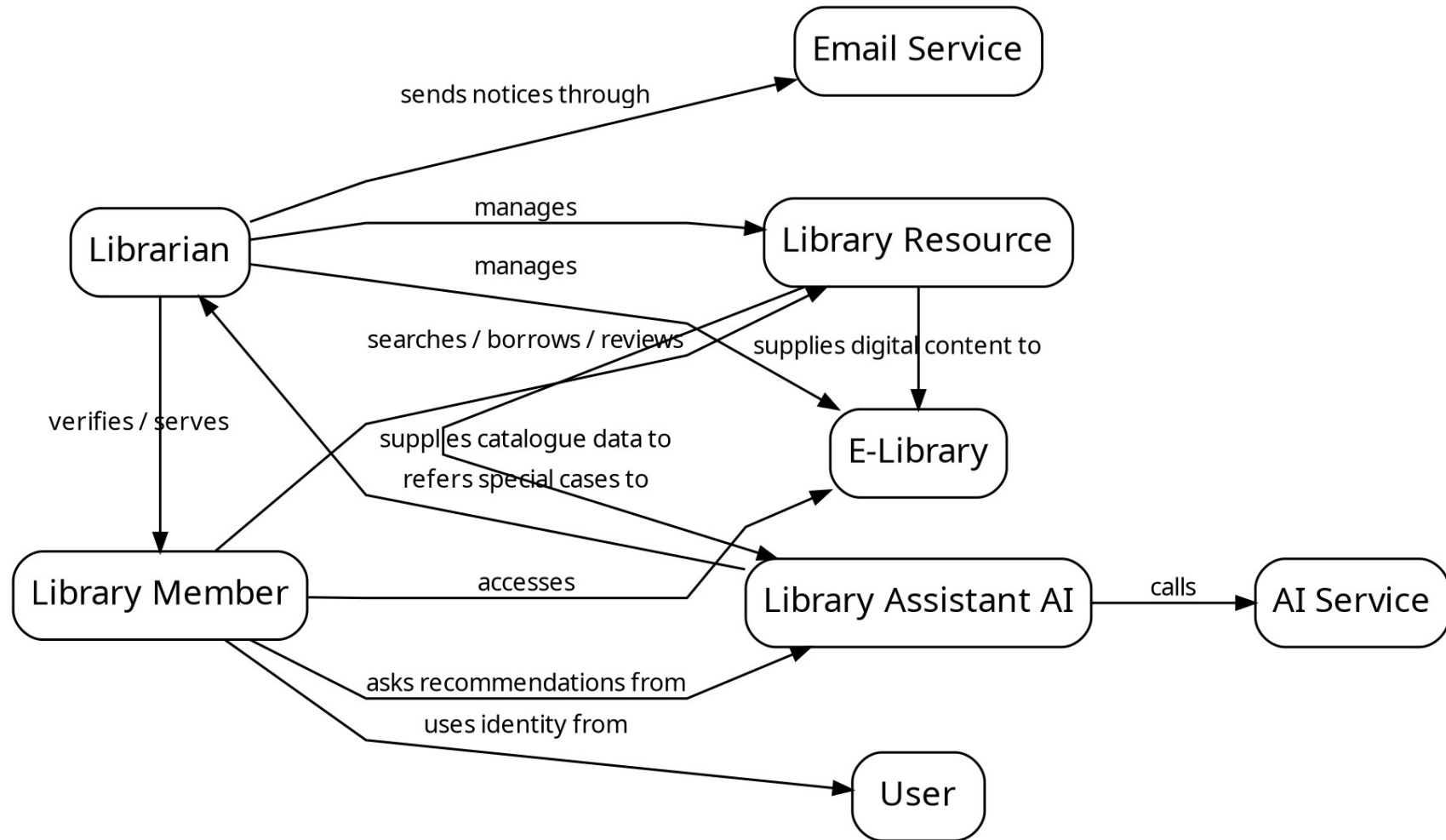
Fig CRC.3: Library Module Collaboration Diagram
