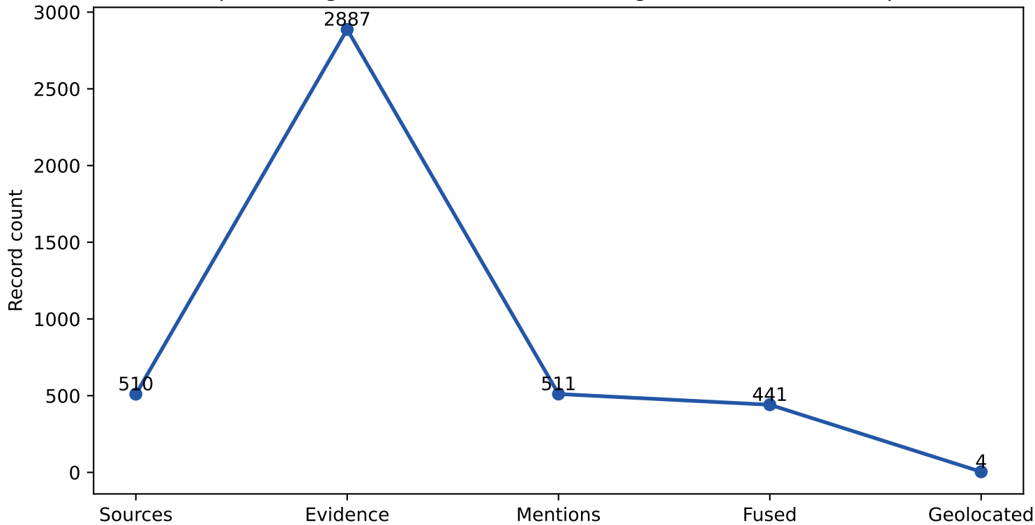
MGeoAI processing funnel (record counts; stages are not attrition-equivalent)
