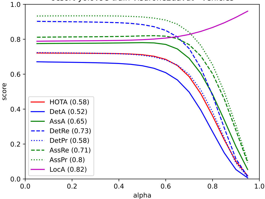
ocsort-yolov9e-train-visdrone2uavdt - vehicles
