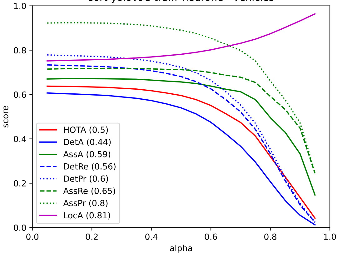
sort-yolov9e-train-visdrone - vehicles
