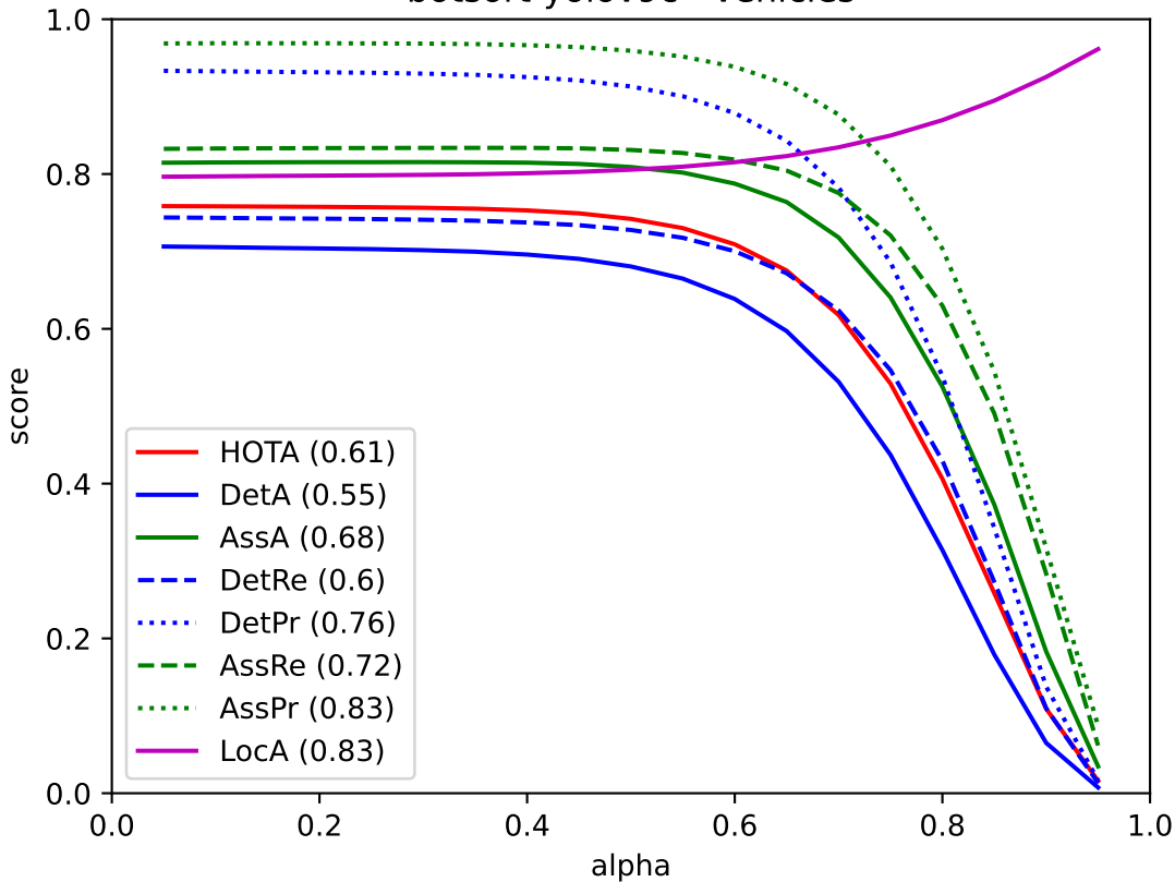
botsort-yolov9c - vehicles
