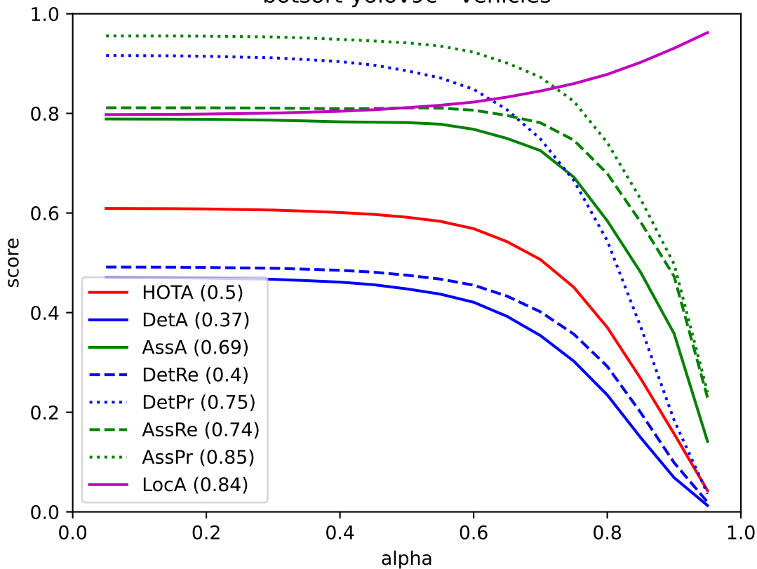
botsort-yolov9c - vehicles
