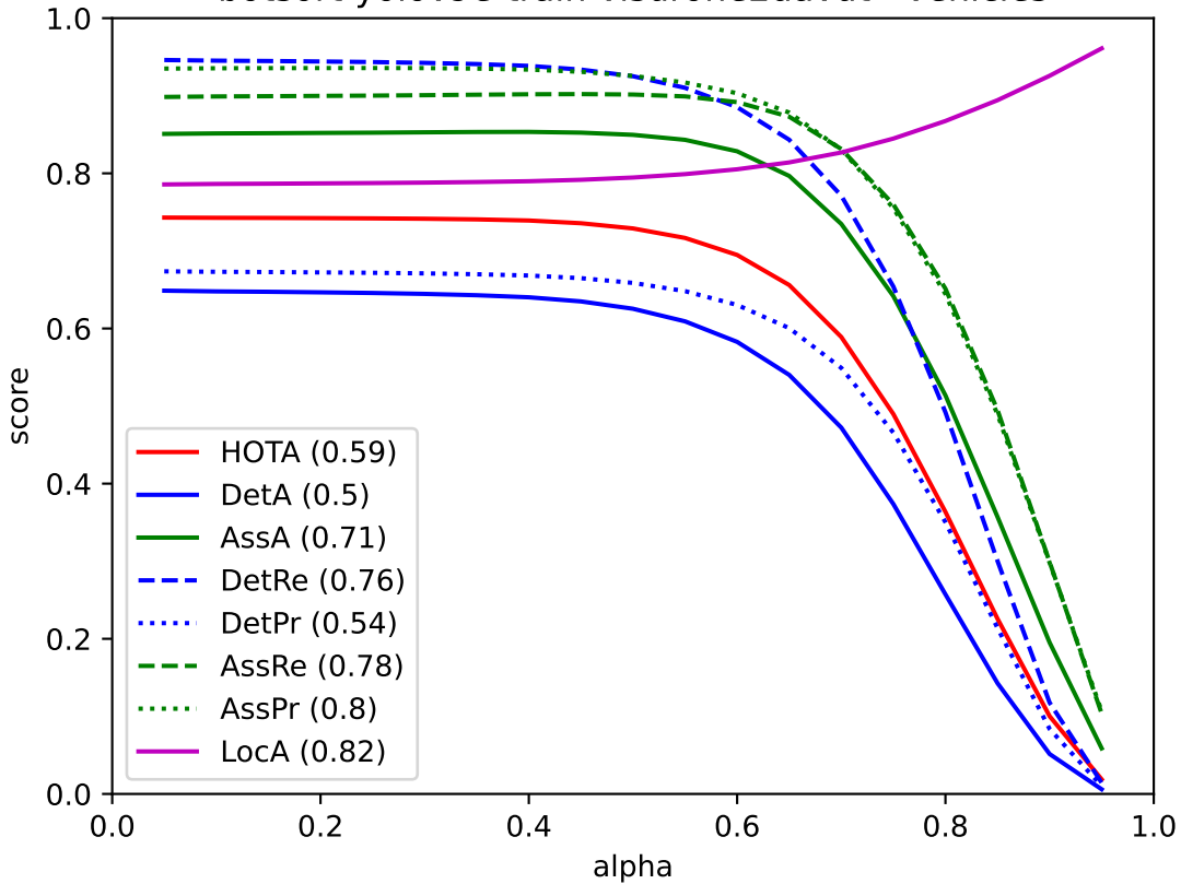
botsort-yolov9e-train-visdrone2uavdt - vehicles
