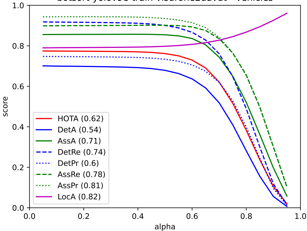
botsort-yolov9e-train-visdrone2uavdt - vehicles
